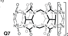
Figure 1. Amino acid sequences of the insulins and model peptides used in this study, and the chemical formula of Q7.
