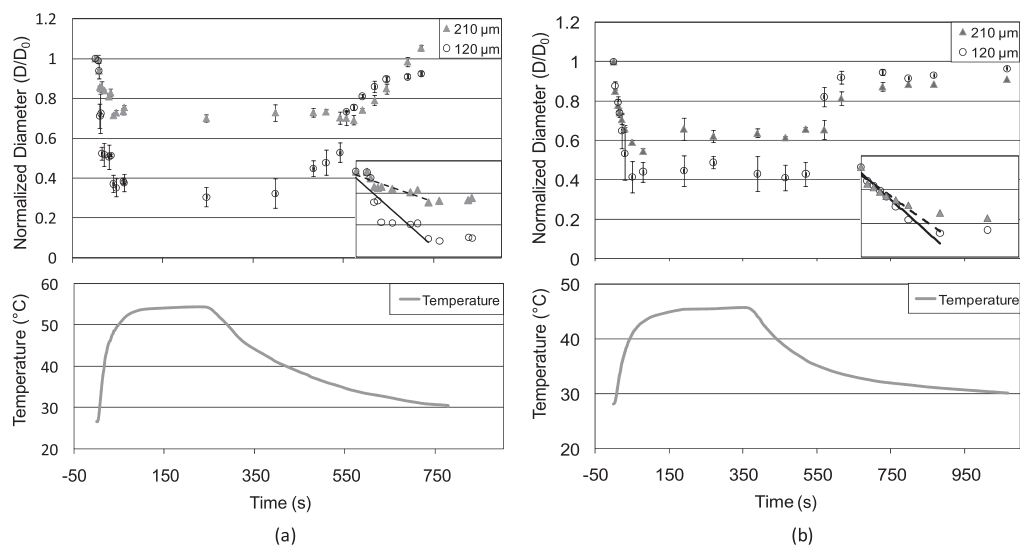
Fig. 4. Dynamic thermal responses of 210- and 120- \mu\text{m} -diameter micropillars made of (a) pure PNIPAAm and (b) nanocomposite PNIPAAm (1.0 wt% polysiloxane nanoparticle). (Standard deviations were from three samples with similar diameters and are marked on the graph.)
