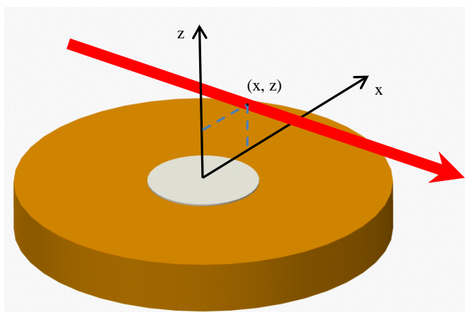
Figure 4. Schematic of the coordinate system centered on the top surface of the central disk. The IR beam was oriented normal to the x - z plane.
