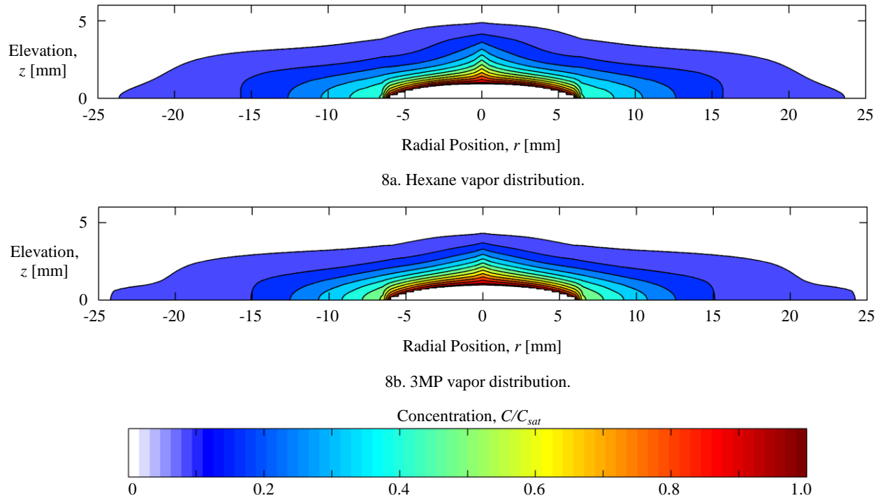
Figure 8. Computed vapor distribution for hexane (8a) and 3MP (8b) in a vertical plane passing through the center of the drop. The vapor concentration is normalized by the saturated value at 22.6°C and an ambient pressure of 96 kPa. The color map indicates the vapor concentration values.
