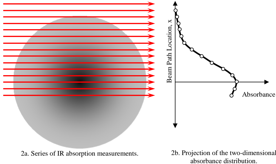
Figure 2. Schematic of a top view of the vapor cloud (grey region) and a series of IR absorption measurements made in a single elevation plane above the drop (Fig. 2a). The resulting distribution of the IR absorption measurements, which is equivalent to a one-dimensional projection of the two-dimensional absorbance distribution, is shown in Fig. 2b.
