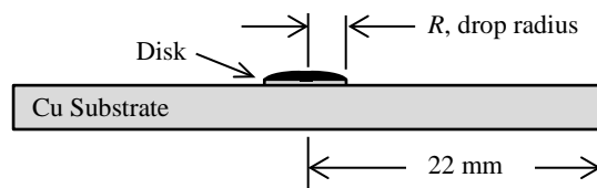
Figure 3. Schematic of a profile view of a sessile drop (black) which covers the surface of a disk at the center of the copper substrate. The drop is attached around the circular periphery of the disk and in this way the drop size is maintained during the majority of the evaporation process.
