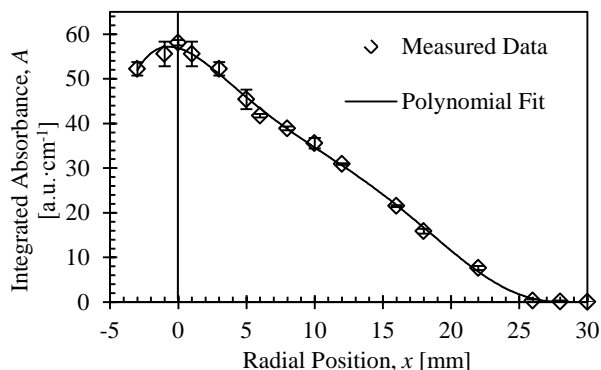
Figure 7. Distribution of integrated absorbance measurements in the z = 3 mm plane for hexane. The data are fitted by a polynomial in order to compute absorbance values with high resolution and at a regular interval. Error bars indicate the standard deviation of the measurements at each radial position.
