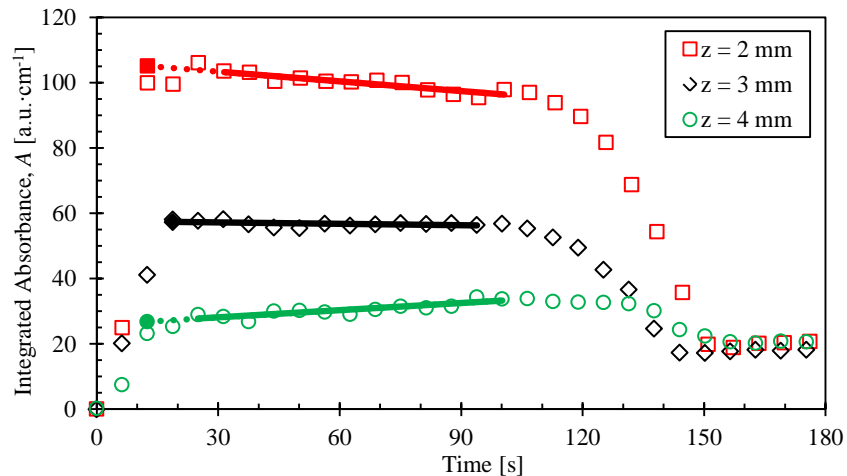
Figure 6. Representative plots of the integrated absorbance as a function of time during a measurement trial. The data was acquired for a hexane drop at x = 0 and z = 2, 3, and 4 mm.
