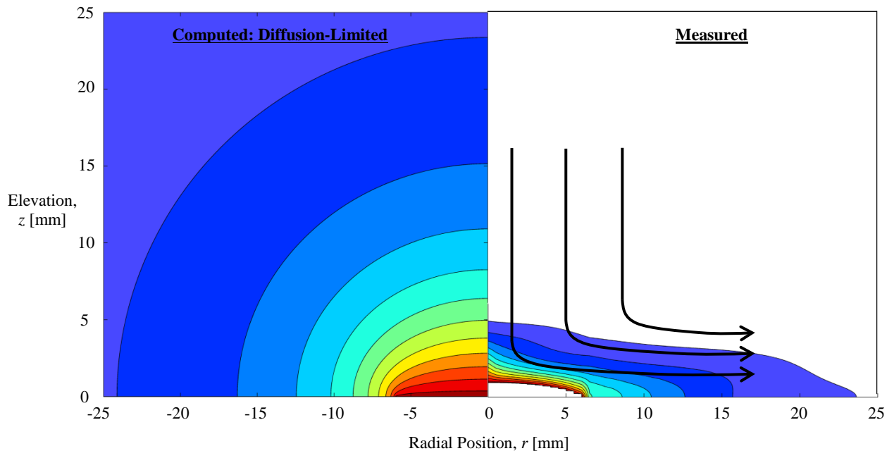
Figure 9. Comparison of vapor distributions for a hexane drop. The distribution for the condition of diffusion-limited vapor transport is given to the left of the central axis and the measured distribution is given to the right of the axis. Hypothesized streamlines of the buoyancy-induced air and vapor flow are shown by the arrows over the measured vapor distribution. Concentration values are given by the color bar in Fig. 8.
