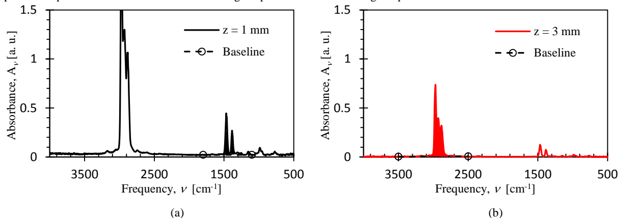
Figure 5. Two absorbance spectra representative of measurements taken at elevations of 1 mm (Fig. 5a) and 3 mm (Fig. 5b) for IR beams passing over the center of the hexane drop. Due to the high vapor concentration directly above the drop at z = 1 mm, the absorbance peak between 3100 - 2800 \text{ cm}^{-1} was saturated and so the peak between 1520 - 1420 \text{ cm}^{-1} was used. For elevations greater than 1 mm, the absorbance peak between 3100 - 2800 \text{ cm}^{-1} was used. The shaded regions represent the integrated absorbance values that were used.
