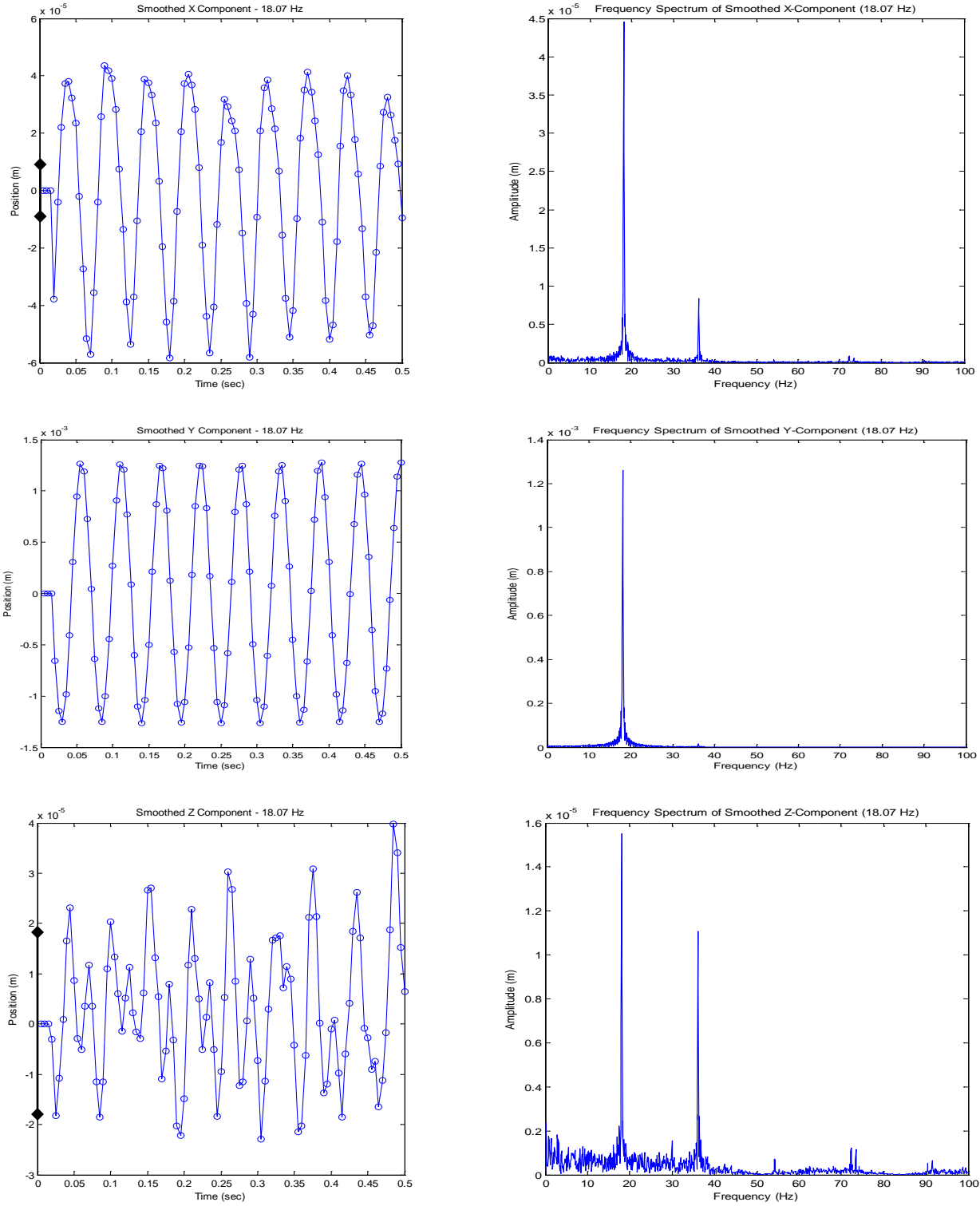
Fig. 12: Position data smoothed through Savitzky-Golay filter for 18.07 Hz oscillation (compare with unfiltered data in Figure 8). 68.3% confidence levels (of \pm 7.92 \mu\text{m} , \pm 14.4 \mu\text{m} , and \pm 18.6 \mu\text{m} respectively for the x-y- and z- directions) are shown to scale on their respective ordinates.
