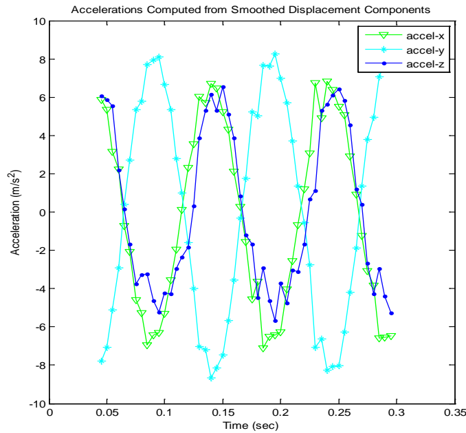
Fig. 18: The accelerations components of the off-axis shaker oscillation computed from the smoothed displacement components showed some noise at each cycle extreme, but otherwise possessed the expected phase-shifted sinusoidal shape. The 68.3% confidence intervals are not resolvable at this scale.
