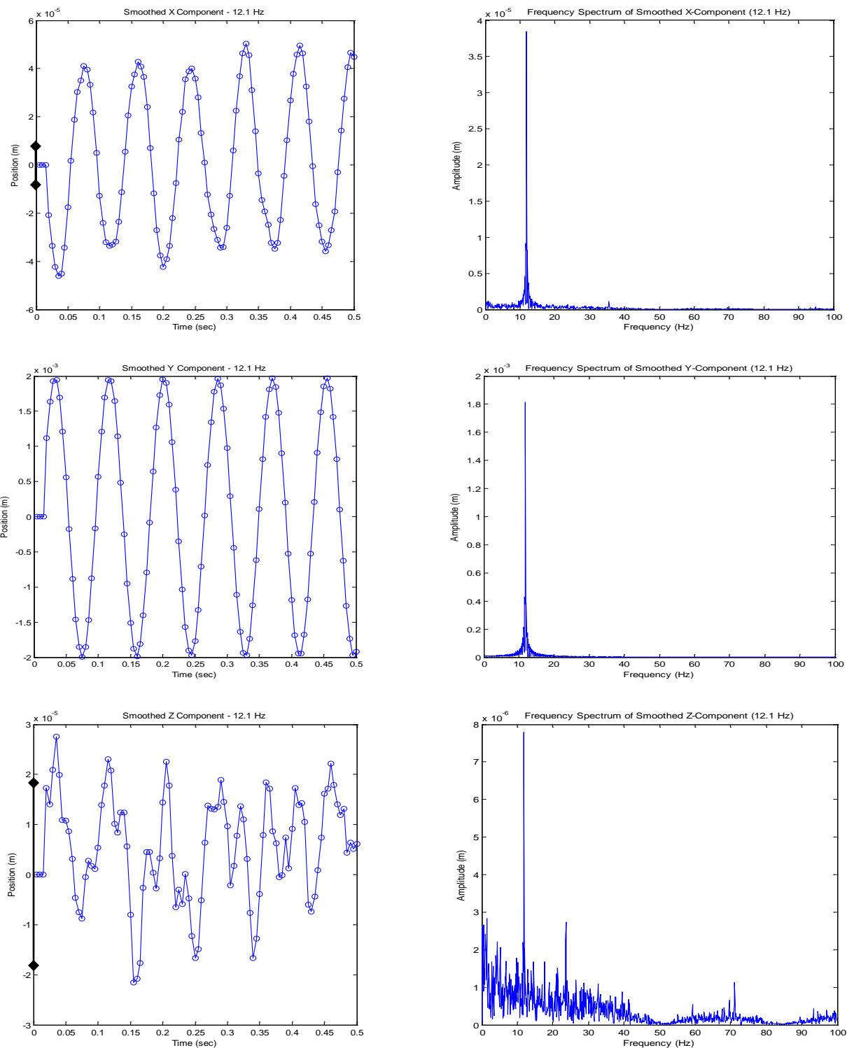
Fig. 11: Position data smoothed through Savitzky-Golay filter for 12.1 Hz oscillation (compare with unfiltered data in Figure 7). 68.3% confidence levels (of \pm 7.92 \mu\text{m} , \pm 14.4 \mu\text{m} , and \pm 18.6 \mu\text{m} respectively for the x- y- and z- directions) are shown to scale on their respective ordinates.
