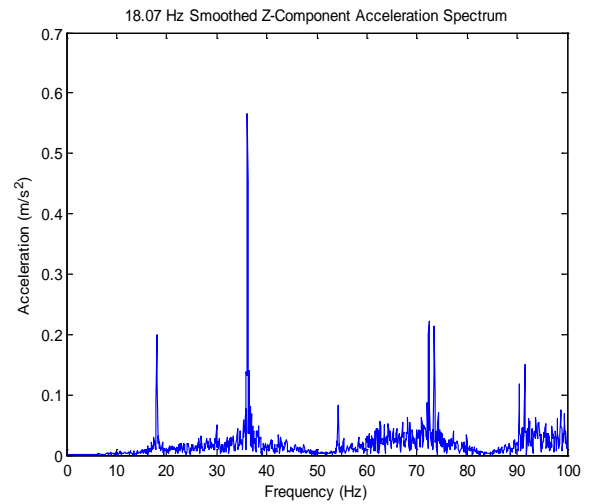
Fig. 14: Acceleration data obtained by twice-differentiating smoothed position data for 18.07 Hz oscillation (from Figure 12); compare with acceleration profile (Figure 10) obtained from unfiltered position data. 68.3% confidence levels (of \pm 0.102 \text{ m/s}^2 , \pm 0.186 \text{ m/s}^2 , and \pm 0.240 \text{ m/s}^2 respectively for the x- y- and z- directions) are shown to scale on their respective ordinates.
