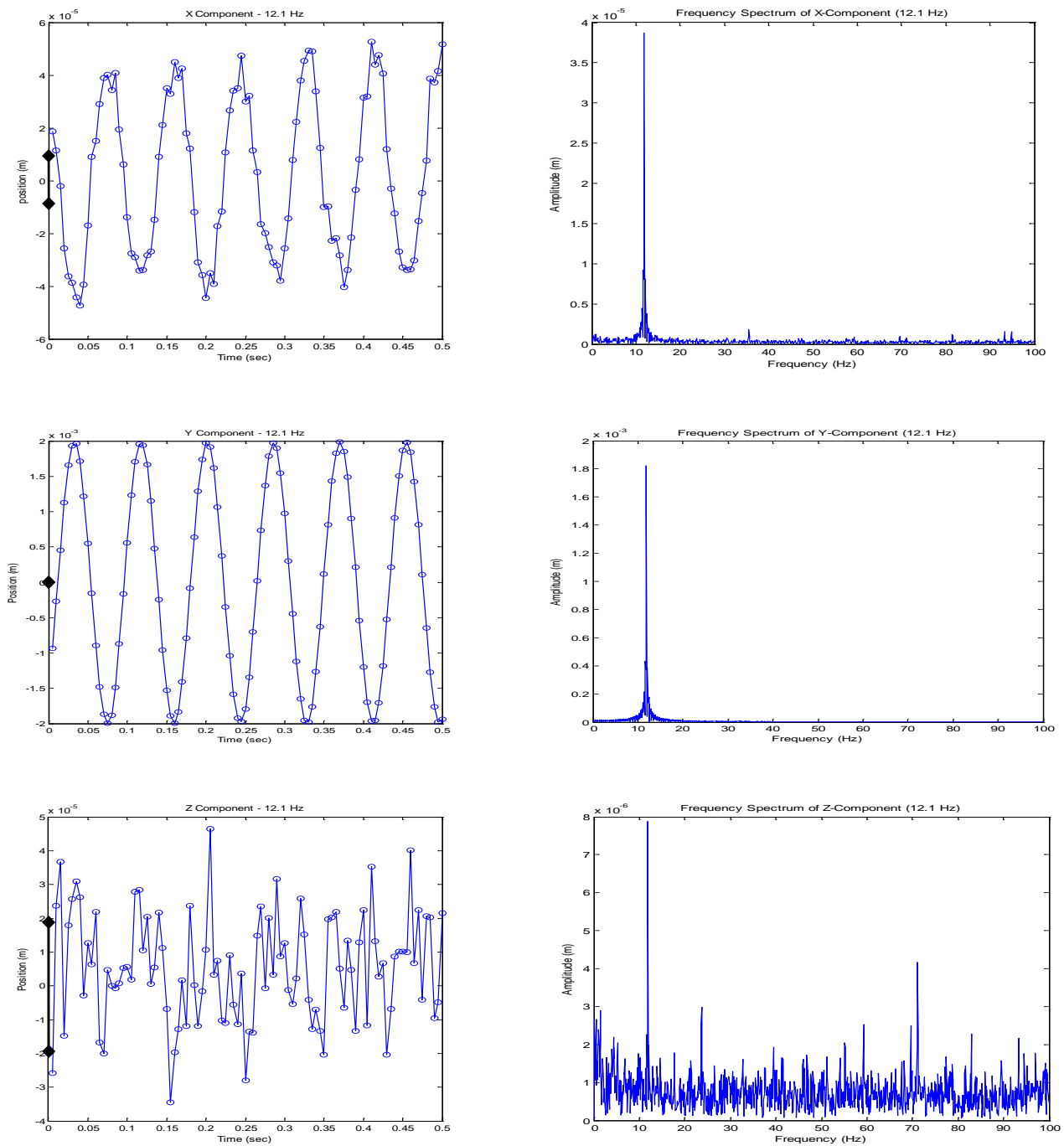
Fig. 7: x-, y- and z-component videogrammetric-based tracking results for a 12.1 Hz y-axis harmonic motion. 68.3% confidence levels (of \pm 7.92 \mu\text{m} , \pm 14.4 \mu\text{m} , and \pm 18.6 \mu\text{m} respectively for the x- y- and z- directions) are shown to scale on their respective ordinates. The tracked motion in the x- and z- directions (non-driven) are almost two orders of magnitude lower than the y-component of motion, indicating good alignment of the reference axis with the vertical. However, the 12.1-Hz component apparent in the top plot does indicate a small component of shaft displacement along the defined x-axis, indicating a slight misalignment between the axis of the shaker and the specified coordinate system. Fourier analysis shows that the spectral content of the z-component also contains the fundamental, even though it is not apparent through simple inspection of the time-domain signal. The z-component of the response also includes a great deal of noise.
