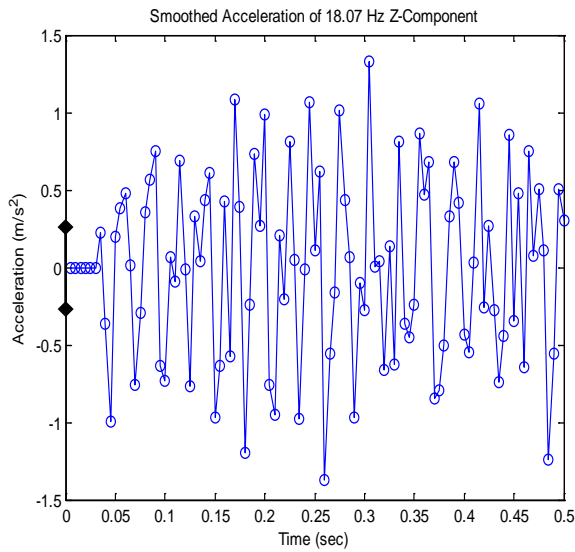
Fig. 14: Acceleration data obtained by twice-differentiating smoothed position data for 18.07 Hz oscillation (from Figure 12); compare with acceleration profile (Figure 10) obtained from unfiltered position data. 68.3% confidence levels (of \pm 0.102 \text{ m/s}^2 , \pm 0.186 \text{ m/s}^2 , and \pm 0.240 \text{ m/s}^2 respectively for the x- y- and z- directions) are shown to scale on their respective ordinates.
