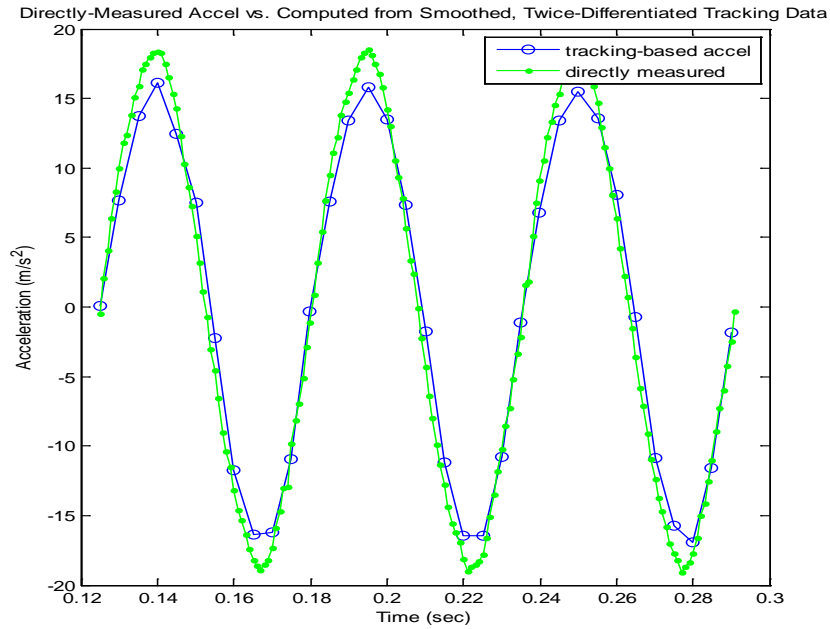
Fig. 16: Directly measured acceleration versus that computed using smoothed, twice-differentiated tracking data (for 18.07 Hz oscillation). The two acceleration measurements track well with each other, except at the vertices where the shaft is changing direction. The 68.3% confidence intervals for neither the video-based nor the accelerometer measurement are resolvable at this scale.
