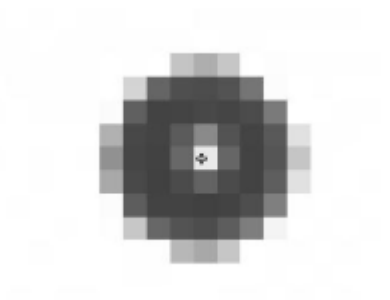
Fig. 2: Zoomed view of a circular, 11-mm black-on-white coordinate-system target, as viewed by one of the videogrammetric cameras. The target diameter corresponds to approximately 9 pixels on the camera's imaging element, equal to a ratio of about 1.22 mm per imaging element pixel. The small "plus" near the center of the image indicates the exact tracking location, which corresponds to the target centroid.
