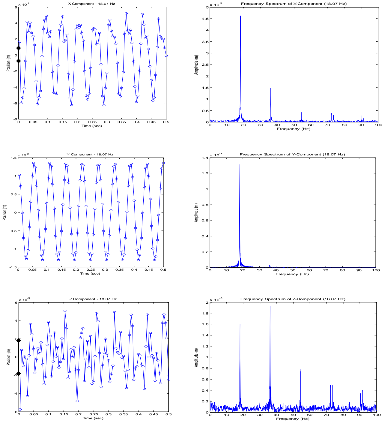
Fig. 8: x-, y- and z-component videogrammetric-based tracking results for an 18.07 Hz y-axis harmonic motion. 68.3% confidence levels (of \pm 7.92 \mu\text{m} , \pm 14.4 \mu\text{m} , and \pm 18.6 \mu\text{m} respectively for the x- y- and z- directions) are shown to scale on their respective ordinates. The tracked motion in the x- and z- directions (non-driven) are almost two orders of magnitude lower than the y-component of motion, indicating good alignment of the reference axis with the vertical. However, the 18.07-Hz component apparent in the top plot does indicate a small component of shaft displacement along the defined x-axis, indicating a slight misalignment between the axis of the shaker and the specified coordinate system. Spectral analysis indicates that both off-axis responses have induced harmonics at integer multiples of the driving frequency. The z-component of the response also includes a great deal of noise.
