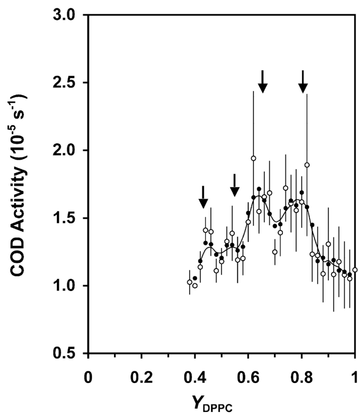
Figure 6. COD activity at 23 °C versus Y_{\text{DPPC}} in DPPC/DLPC/CHOL liposomes for for X_{\text{CHOL}} = 0.40 . The data represent averages of measurements from 11 parallel and independently prepared liposome preparations. See legends of Figure 2 for other details.
