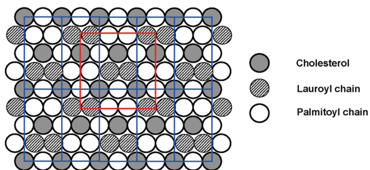
Figure 7. Proposed organizations of simultaneous cholesterol and acyl chain superlattices in DPPC/DLPC/CHOL bilayers at the theoretical critical compositions of X_{\text{CHOL}} = 0.40 and Y_{\text{DPPC}} = 0.67 . Ten unit cells (blue squares) of Cholesterol SL (CHOL/PC-SL) in centered rectangular symmetry and one unit cell (red square) of Phospholipid SL (DPPC/DLPC-SL) also in centered rectangular symmetry with the double-chains of DLPC as the host are shown.
