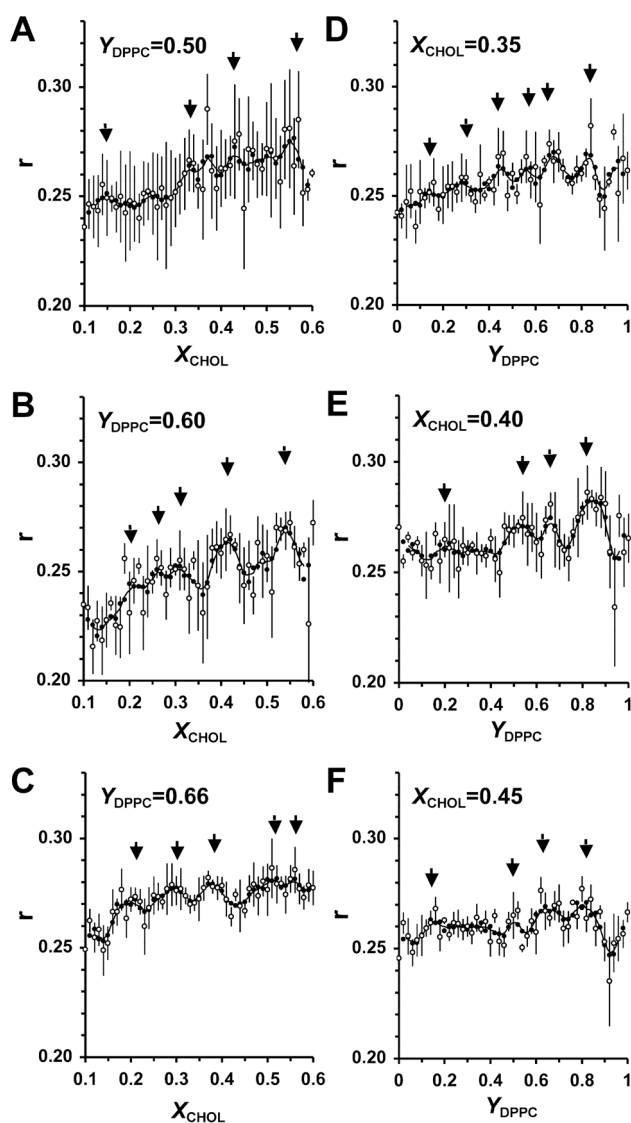
Figure 2. Steady-state anisotropy r of DPH-PC in DPPC/DLPC/CHOL bilayers versus CHOL/lipid mole ratio ( X_{\text{CHOL}} ) (left column) plots at 23 °C for a fixed DPPC/PC mole ratio ( Y_{\text{DPPC}} ) of 0.50 (A), 0.60 (B), and 0.66 (C). The r versus Y_{\text{DPPC}} (right column) plots at 23 °C for a fixed X_{\text{CHOL}} of 0.35 (D), 0.40 (E), and 0.45 (F) are also shown. Raw averaged data from parallel samples ( \circ ), one-pass three-point moving averages ( \bullet ) and two-pass three-point moving averages (line) are presented. The arrows indicated the identified peaks (see Materials and Methods). Bars indicate standard errors. The data represent averages of measurements from three ( N = 3 ) parallel and independently prepared liposome preparations for all samples except the plot with a fixed X_{\text{CHOL}} of 0.40 in which N = 4 .
