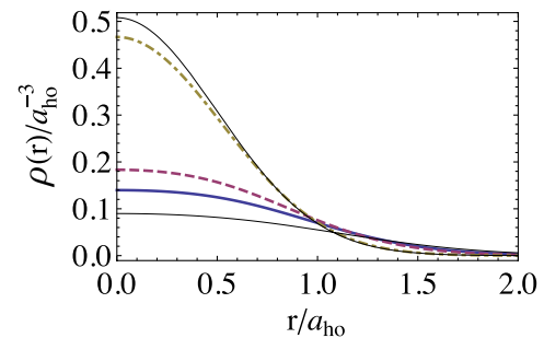
Figure 20. Single-particle density profiles for interaction strength across the crossover. Thick curves correspond to numerical results: a = -a_{ho} (solid curves), a = \pm\infty (dashed curves) and a = 0.1a_{ho} (dash-dotted curves). Thin curves correspond to analytic limiting solutions: non-interacting four-fermion prediction (less peaked), dimer-dimer solution in the BEC limit (more peaked).
