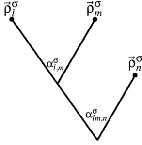
Figure A5. The hyperspherical tree used to parameterize the hyperangular coordinates in the four-fermion problem is shown. See chapter 2 or [97] for details.
