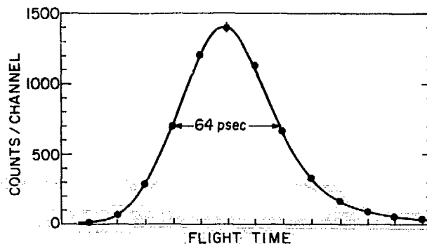
Fig. 7. Measured time spectrum of the bunched ^{160} beam for the maximum detector-bias voltage (250 V). The incident-phase range was selected by limiting the final energy to values near the incident energy.
