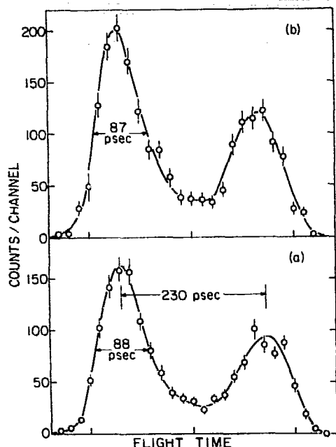
Fig. 6. Measured time spectrum of the bunched ^{160} beam when the detector bias voltage was low (70 V). Curve (a) gives the results obtained when the incident-phase range was selected by limiting the final energy to values near the incident energy. Curve (b) was obtained when the chopper selected the incident-phase range.
