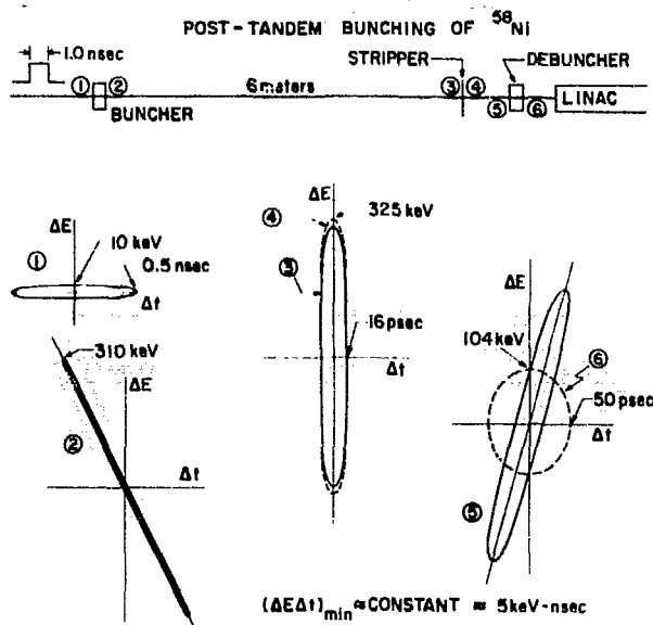
Fig. 3. Bunching process in the post-tandem region for ^{58}\text{Ni} ions and a foil stripper in a tandem with a 10-MV terminal.
