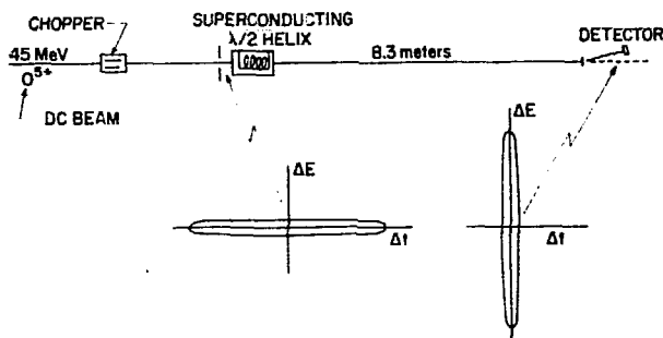
Fig. 4. Schematic of the bunching experiment.
