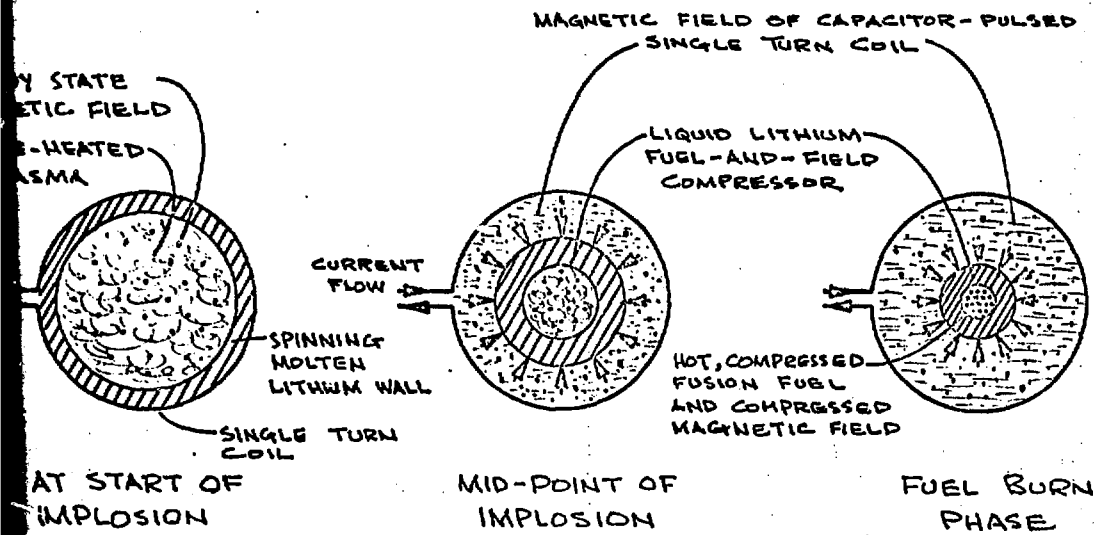
IMPLOSION AND BURN OF FUSION FUEL (END CROSS SECTION)
