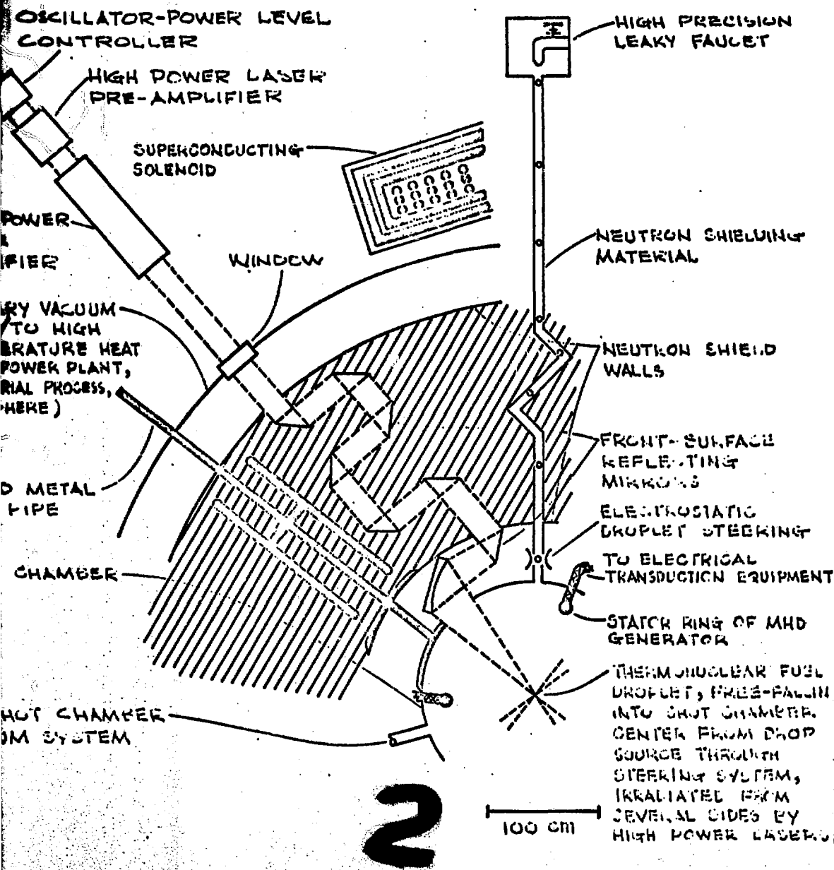
SECTION OF CONCEPTUAL DESIGN OF 1000 MW-SCALE LASER FUSION ELECTRICAL POWER PLANT WITH DIRECT CONVERSION OF EXPLOSION ENERGY TO ELECTRICITY (100 MICROEXPLOSIONS PER SECOND)
