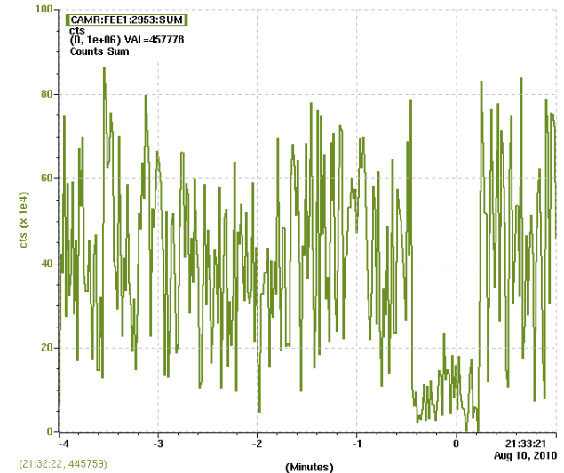
Figure 16: Gas Detector Signal showing SHAB output while Laser Heater is deactivated (low intensity section).
