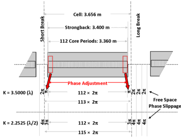
Figure 3: LCLS Undulator Phase Scheme: For the regular strength, the Cell length of 3.656 m is defined as the distance over which the phase slippage is exactly 113 \times 2\pi rad. The transition between the 112 core period and the Cell boundary is tuned to be \pi rad for each undulator. The Break length is designed to be a multiple of \lambda_u (K_1^2/2 + 1) for which 2\pi rad phase slippage occurs in free space. With the larger gap, the transition phase is adjusted to be 3\pi rad.
