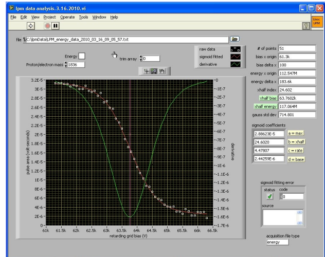
Figure 4. The analyzed data from an energy scan on with a 117.06MeV beam.
