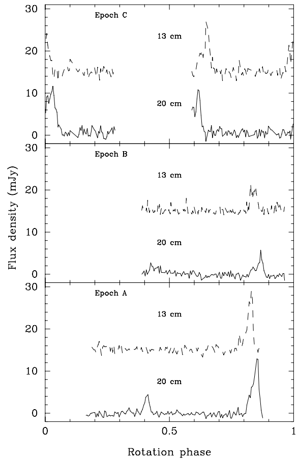
Figure 2. Illustration of the varying pulse phases with respect to the ephemeris of Pyper et al. (1998). The pulse profiles from Epochs A, B and C are shown in the bottom, middle and top panels, respectively. The 13-cm Stokes V pulses (dashed lines) are placed at +15 mJy to differentiate them from the 20-cm Stokes V pulses (solid lines).
