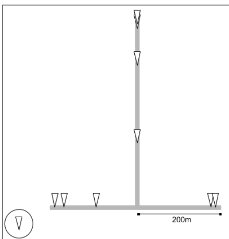
Figure 8. DSA-10 antenna locations. Nine of the antennas are placed on the pre-existing “T” (Tee) shaped infrastructure at the observatory, an \approx 430 (NS) \times 400 (EW) layout, with a tenth (circled) located to the west, providing a long baseline to aid in localisation. The figure is to scale, with the exception of antenna 10, which is located 990 m west, and 217 m south of the center of the Tee.
