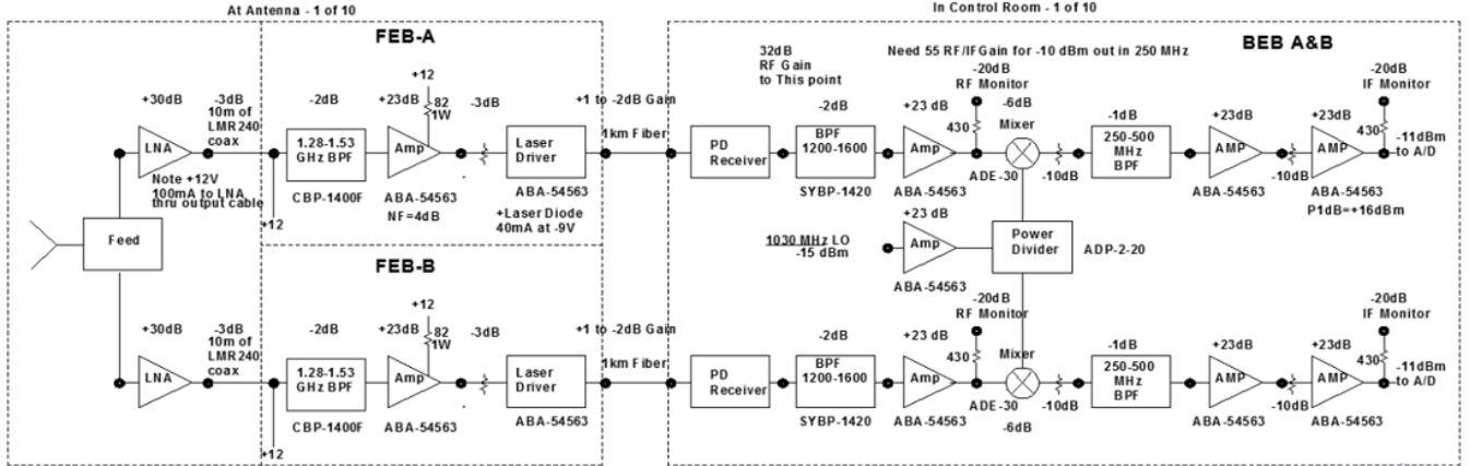
Figure 3. Analogue system receiver chain. The are four main areas of the analogue system. (1) Feed, a dual polarisation 1.28-1.53 GHz feed. (2) LNA, 1300-1700 MHz off the shelf LNA providing 30 dB of gain. (3) FEB, a custom filter, amplifier and optical conversion box for transmitting data back to a central control room. (4) BEB, a custom design to return the optical signal back to RF, filter and down-convert to the 250-500 MHz IF presented to the digital system.
