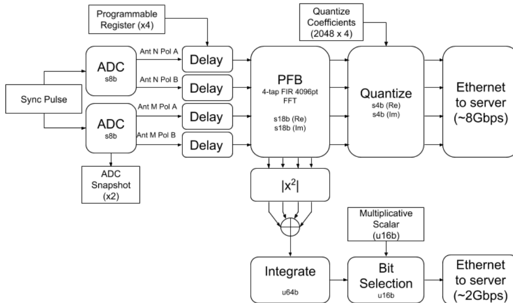
Figure 5. FPGA internals. As the inputs from the BEB are split over multiple SNAPs, each containing ADCs and FPGAs, the system is synchronized via a 1 PPS. A programmable delay block is available for each input to coarsely remove the delays between the different antennas. After being transformed to the frequency domain via PFB, an incoherent sum of each input to the SNAP is made for transmission to a central server. The non-integrated data stream is re-quantized and transmitted at full rate to a separate set of servers (one per SNAP) for buffering, to be written to disk if a candidate is detected in the incoherent sum
