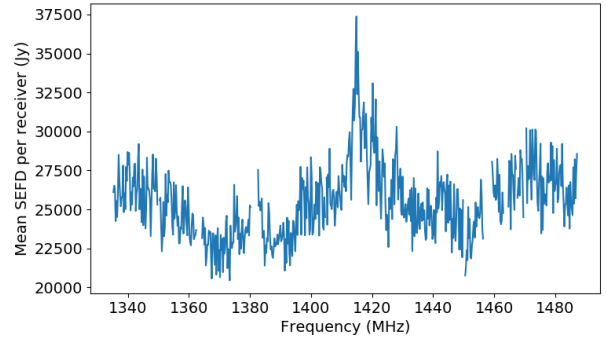
Figure 10. Mean per-antenna system-equivalent flux density (SEFD) estimated using the bright calibrator source 3C409, assumed to have a mean flux density of 13.7 Jy in the observing band but observed 1.5 deg off-boresight. Channels affected by RFI have been excised.
