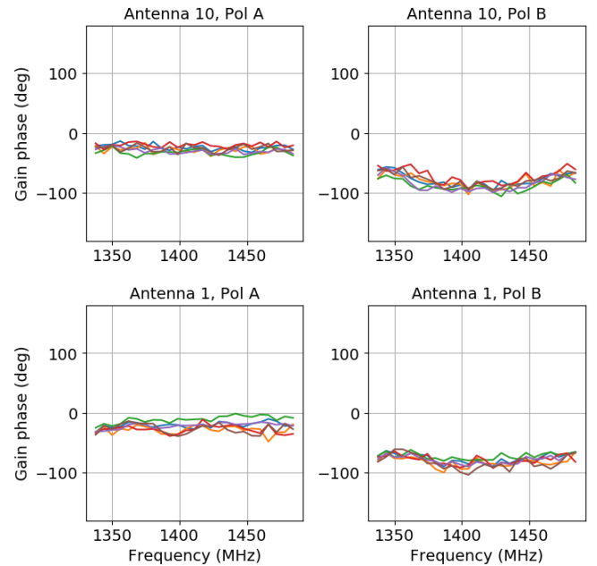
Figure 11. Phases of the complex gains in each polarisation for two antennas estimated using calibrators spaced by approximately 12 hours over three days. Antenna 10 is the sole antenna not sited on the Tee infrastructure, and antenna 1 is the northernmost antenna of the array.
