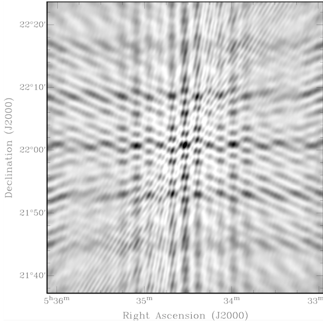
Figure 9. Simulated interferometric point-spread function of DSA-10 at the declination of the Crab pulsar.
