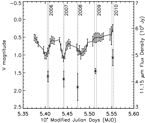
FIG. 5.— Plot of the visual magnitude, and total 11.15\ \mu\text{m} flux density, of Betelgeuse over the period 2006–2010. The visual magnitude measurements, joined by a solid line, are 30-day averages of data obtained from the AAVSO online archive. The 11.15\ \mu\text{m} flux density measurements, also listed in Table 1, are shown here as crosses. The timespans of each ISI observing epoch are bounded by vertical dotted lines.
