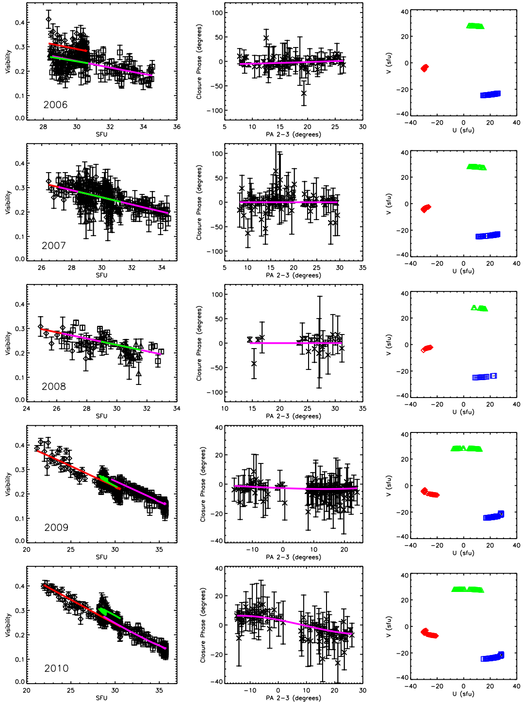
FIG. 1.— Plots of the ISI measurements of Betelgeuse from 2006–2010. The left panels show visibilities, the center panels show closure phases, and the right panels show UV coverages, for each observing epoch (2006 to 2010 from top to bottom). The visibilities for each baseline, denoted 1-2, 2-3 and 3-1, are depicted by diamonds, triangles and squares respectively (note that the spatial frequency ranges vary from year to year). The fitted model visibilities (Table 2) are shown as red, green and magenta lines for baselines 1-2, 2-3 and 3-1 respectively, and as magenta lines for the closure phases. The closure phases are plotted against the position angle, East of North, for baseline 2-3. In the plots of the UV coverage, baseline 1-2 is represented by red diamonds, baseline 2-3 is represented by green triangles, and baseline 3-1 is represented by blue squares.
