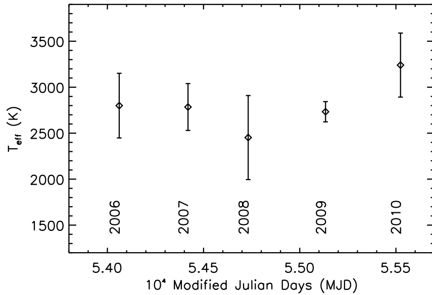
FIG. 3.— The effective temperature of the apparent 11.15\ \mu\text{m} stellar disk of Betelgeuse for each ISI observing epoch in the present work.
