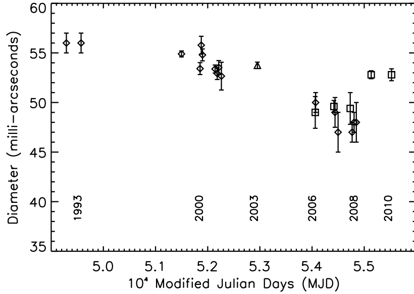
FIG. 2.— The UD diameter of Betelgeuse at 11.15\ \mu\text{m} measured using the ISI over the period 1993–2010. Data between 1993 and 2009, plotted as diamonds, are taken from Townes et al. (2009), and additional data between 2006 and 2010, plotted as squares, are from the present work. The 11.15\ \mu\text{m} UD diameter measurement of Perrin et al. (2007), obtained in 2003 with the VLTI, is plotted as a triangle. The Modified Julian Day (MJD) corresponding to a given Julian Day (JD) is \text{MJD}=\text{JD}-2400000.5 .
