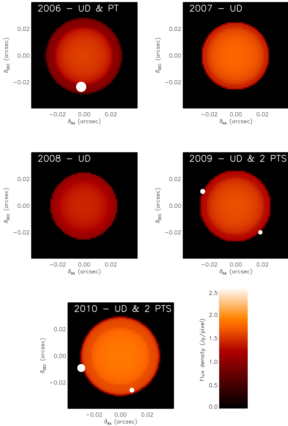
FIG. 4.— Representations of the photosphere-and-layer model intensity distributions fitted to ISI observations of Betelgeuse for each observing epoch in the present work. The locations of the fitted point sources are shown as white disks: the areas of the disks scale linearly with their intensities. The visibility model fitted to each dataset is specified at the top of each image: the 2006 data were fit with a UD and single point source, the 2007 and 2008 data were only fit with a UD, and the 2009 and 2010 data were fit with a UD and two point sources. The color bar shows the flux density per pixel for each color depicted, and each pixel is 1.2 \times 1.2 milli-arcseconds in size.
