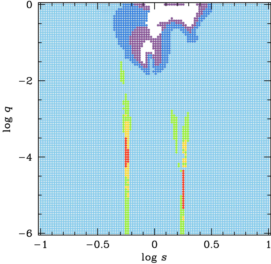
Fig. 2.— \Delta\chi^2 map in (\log s, \log q) space drawn from the grid search. The space is equally divided on a (100 \times 100) grid with ranges of -1 < \log s < 1 and -6 < \log q < 0 , respectively. The contour is color coded by (red, yellow, green, light blue, blue, purple) for \Delta\chi^2 < [(1n)^2, (2n)^2, (3n)^2, (4n)^2, (5n)^2, (6n)^2] , where n = 20 .
