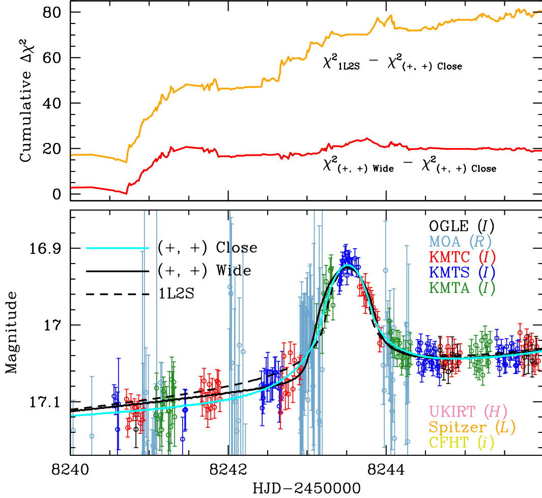
Fig. 6.— Cumulative distributions of \Delta\chi^2 in the anomaly region. In the upper panel, the red and orange curves represent the \chi^2 differences between the (+, +)_{\text{Wide}} and (+, +)_{\text{Close}} solution and between the 1L2S and (+, +)_{\text{Close}} solution, respectively. In the lower panel, the cyan, black solid, and black dashed curves plotted over the data are the model curves based on the (+, +)_{\text{Close}} , (+, +)_{\text{Wide}} , and 1L2S solution, respectively.
