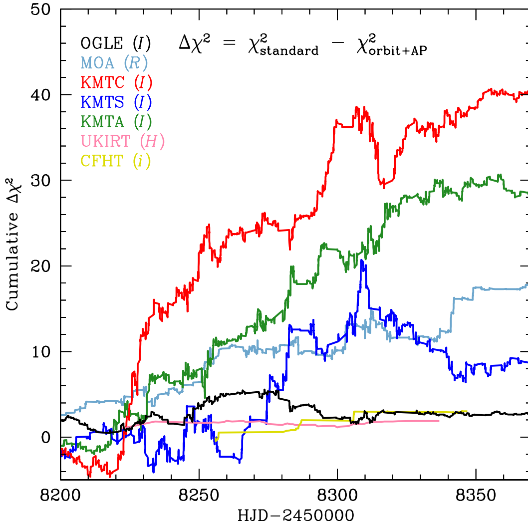
Fig. 4.— Cumulative distribution of \Delta\chi^2 between the standard and the “orbit+AP” solution derived from the ground-based observations. Note that the diagram is constructed using the best-fit model from the (+, +)_{\text{close}} caustic topology.
