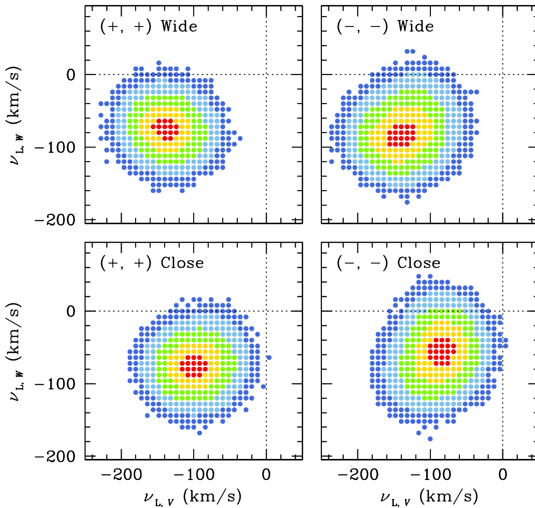
Fig. 8.— Distributions of lens projected velocities \nu_L estimated from the four solutions. The color notation is same as in Figure 5. Note that the reference frame is the local standard of rest (LSR).
