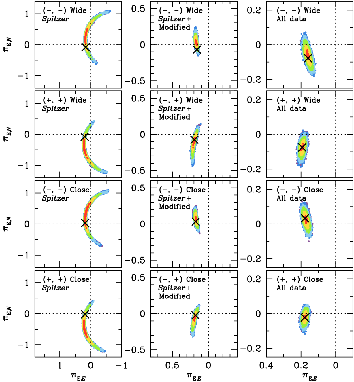
Fig. 5.— \chi^2 as a function of microlens parallax for different data sets. The left, middle, and right four panels show the derived \Delta\chi^2 maps in the (\pi_{E,N}, \pi_{E,E}) plane based on the Spitzer data, Spitzer +modified ground data, and all data sets, respectively. In each panel, the black cross marks the location of \pi_E listed in Table 1 and 2. Except that here n = 1 , the color coding is same as in Figure 2. Note the different scales in the three columns.
