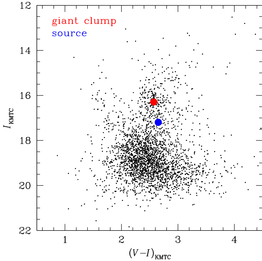
Fig. 7.— Instrumental Color-magnitude diagram of stars around OGLE-2018-BLG-0596 (within 120'' ) based on the KMTC star catalog. The red and blue dots indicate the positions of the giant clump centroid (GC) and the microlensed source, respectively.
