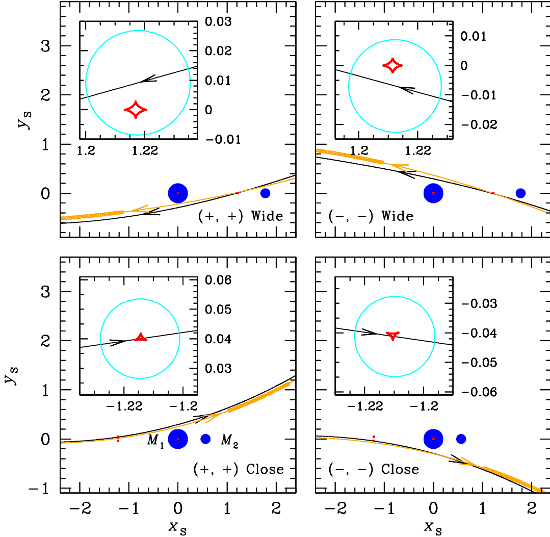
Fig. 3.— Caustic geometries of the four solutions of OGLE-2018-BLG-0596. In each panel, the orange curve is the Spitzer -viewed source trajectory, while the black curve is the Earth-viewed source trajectory. The orange circles are the source positions at the times of Spitzer observation. These are not shown to scale in order to avoid clutter. The red closed curves are the caustics, and the two dark blue dots are the binary lens components. The inset shows the enlarged view of the small planetary caustic at the time of the source’s caustic envelopment. The cyan circle represents the source radius \rho of the best-fit solution (cf. Table 1 and 2).
