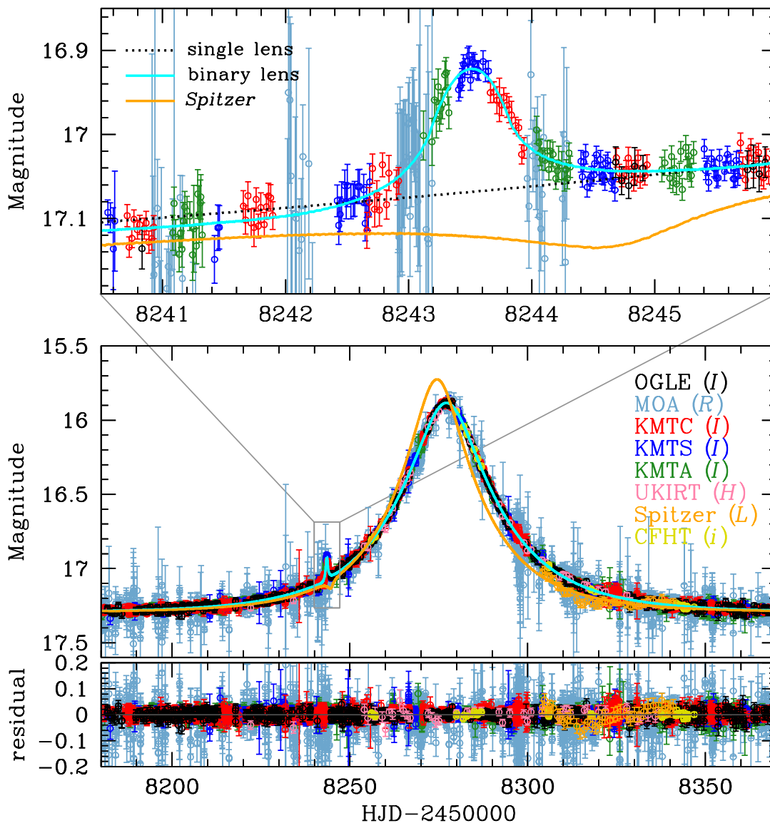
Fig. 1.— Light curve of OGLE-2018-BLG-0596. The upper panel shows the enlarged view of the anomaly centered at \text{HJD}' \sim 8243.5 . The cyan and orange curves are the best-fit model curves for the ground- and space-based observations, respectively. The black dotted curve is the model curve obtained from the 1L1S interpretation.
