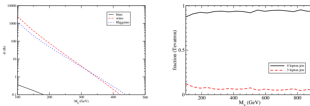
Figure 23. Left: The cross-sections for electroweak-ino production at the Tevatron. We have included both LSP pair production and, in the case of wino and Higgsino LSP, the production of closely degenerate states, as a function of M_\chi . We choose the squark mass to be 750 GeV. Right: the fraction of events with 3 and 4 lepton jets within the central region |\eta| < 2.4 .
