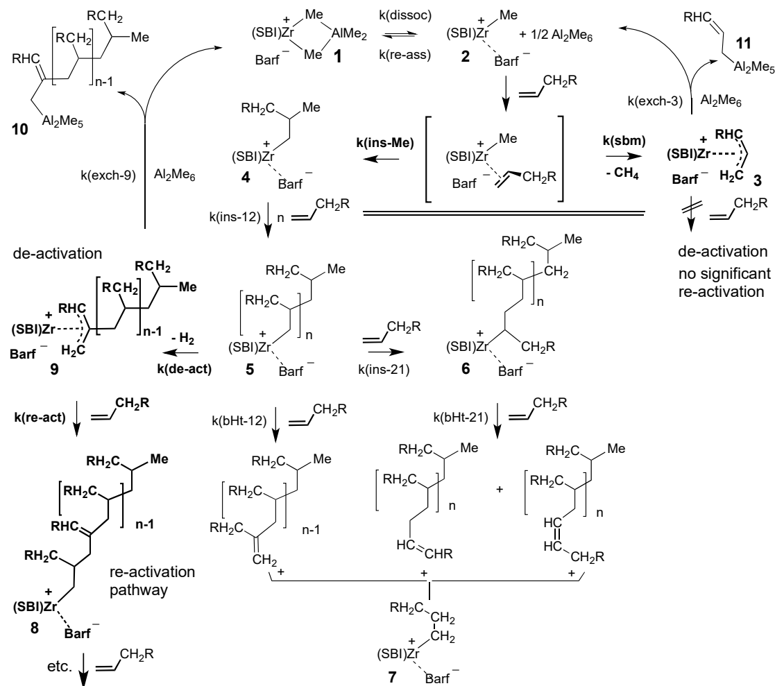
Scheme 1. Selected reaction participants and products proposed for the polymerization of 1-hexene ( R = n -propyl) by the pre-catalyst SBIZr(\mu-Me)_2AlMe_2^+ ( C-0 , complex 1 ): Zr-alkyl and -polymeryl species of spectral type C-1 (complexes 4-8 ), Zr-allyl species of spectral type C-2 (complexes 3 and 9 ), polyolefins with Al-capped allylic chain ends formed from complexes 3 and 9 (Al-complexes 10 and 11 ) and polyolefin chains released from Zr-polymeryl species by \beta -H transfer. The non-observable initiation intermediate, which might react either by sigma-bond metathesis to form complex 3 or by olefin insertion to form complex 4 is shown in heavy square brackets. Omitted for clarity are diastereomers of Zr-allyl complexes 3 and 9 as well as polyolefin chains with Al-capped saturated chain ends formed by methyl- vs. -polymeryl exchange of Al_2Me_6 with Zr-alkyl and -polymeryl complexes 4-8 ( Barf^- = B(C_6F_5)_4^- ).
