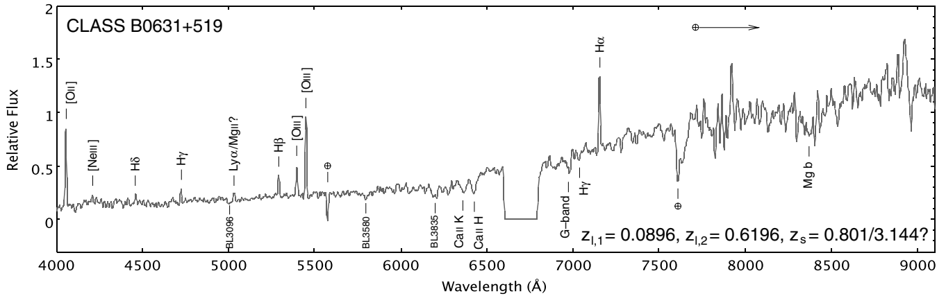
Figure 4. The optical spectrum of CLASS B0631+519 taken with the W. M. Keck-I Telescope on 2001 November 16 using LRIS. Eight emission lines from a lensing galaxy at z_{1,1} = 0.0896 \pm 0.0001 and seven absorption features from a second lensing galaxy at z_{1,2} = 0.6196 \pm 0.0004 have been detected. The redshift of the background source is unknown although a weak emission line at 5040 \text{ \AA} may be either Ly\alpha or Mg\ II . The data above 7700 \text{ \AA} are very noisy and are included only to show that the second deflector is an early-type galaxy. The relative flux has units of 10^{-17} \text{ erg cm}^{-2} \text{ s}^{-1} \text{ \AA}^{-1} . The spectrum has been smoothed using a boxcar of 10 \text{ \AA} .
