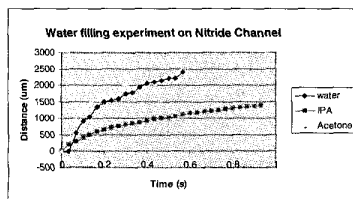
Figure 5: The position of a capillary meniscus vs. time of different liquids filling into a silicon nitride microchannel.
