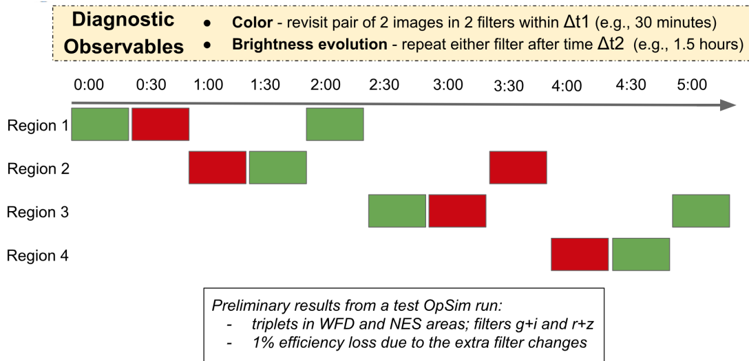
Figure 3: An example Presto-Color cadence with two alternating filters cover regions of sky to obtain three observations per region with appropriate time gaps to measure lightcurve color and shape.
