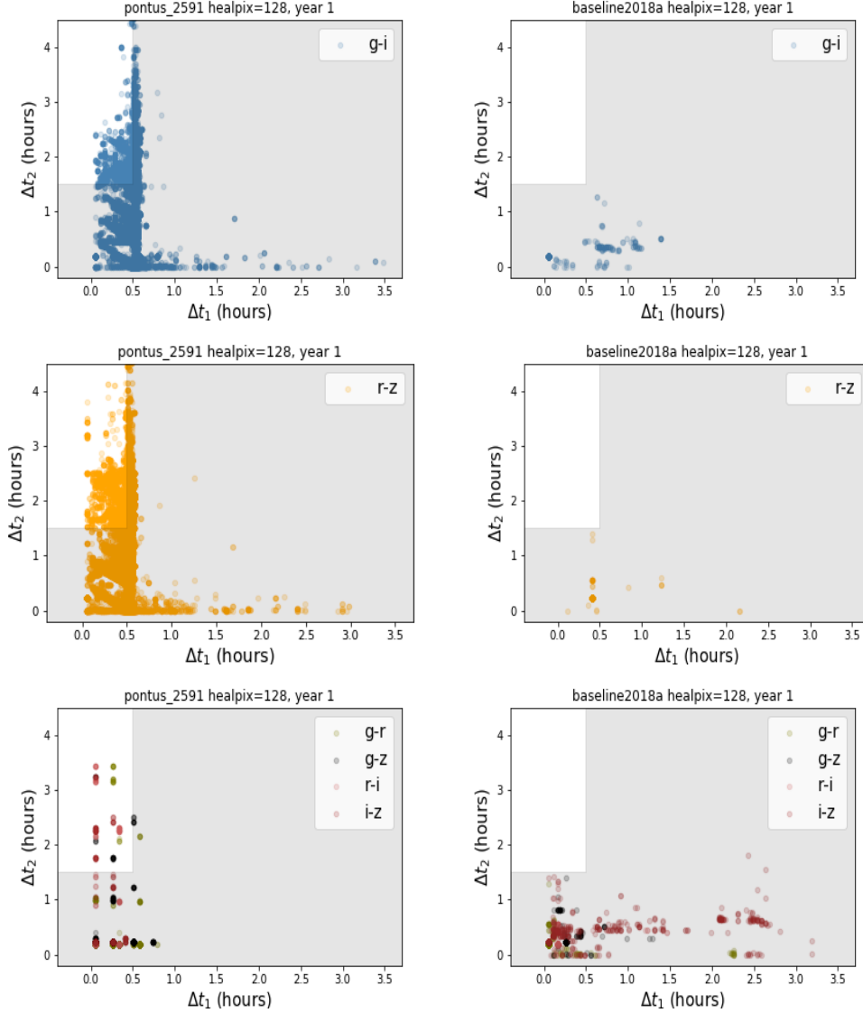
Figure 4: The results of our diagnostic metric, threeVisitsWColorMetric , that checks for fields that were observed 3 times in a night with 2 filters (as labeled) satisfying the constraints on \Delta T_1 and \Delta T_2 . We show results for 1-year of pontus_2591 (our Presto-Color test run; left), and baseline2018a LSST observations (right). All HEALpix “fields” that met the conditions of our metric are shown as points, colored by the filter pair f_1 - f_2 . The x -axis is the time between visits in the two different filters (which provide color; \Delta T_1 ), and the y -axis is the time between visits in the same filter (which provides slope; \Delta T_2 ). The target area for our science is the white region, where \Delta T_1 < 0.5 and \Delta T_2 > 1.5 hours, such that both color and brightness evolution can be measured, although there is no hard cutoff at 30 minutes in \Delta T_1 , so observations just to the left of our target region are valuable, and observations at a larger \Delta T_2 within the same night are preferred. In pontus_2591 20 thousand observations in year 1 satisfy our constraints strictly ( \Delta T_1 < 0.5 and \Delta T_2 > 1.5 ) in g-i and over 40 thousand in r-z . Very few HEALpix fields in the baseline2018a OpSim have observations in triplets in 2 filters and none that satisfy our constraints.
