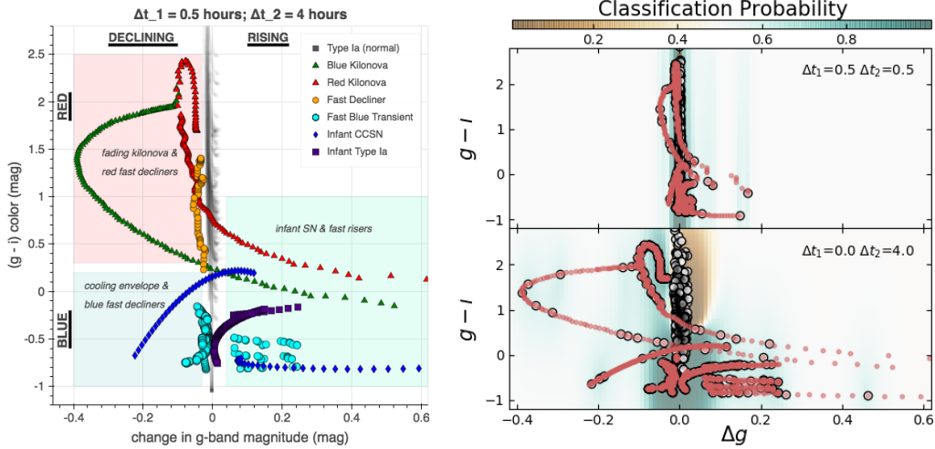
Figure 2: Left : Phase space plot showing separation between classes of transients in observed color and intra-night magnitude change. This fiducial plot assumes observations are obtained in g - and i -band filters within 30 minutes ( \Delta T_1 ) and a second g -band observation is obtained 4 hours ( \Delta T_2 ) later at a range of epochs in each transient’s evolution. Rising light curves correspond to positive magnitude changes. Observations of our four exemplar types of fast transients/phases are plotted in color. For kilonovae, we include models of GW170817 both with and without the early blue component. “Infant” SN correspond to observations within the first 5 days post-explosion. The infant core-collapse SN found in the declining portion of the plot is the rapidly-fading component of the cooling envelope emission observed in SN2016gkg (see Fig 1). We also show a population of normal Type Ia SN between -7 and +20 days of maximum light—at a range of redshifts—representing slower evolving transients from which we wish to distinguish our transients of interest. Right : A classifier can be trained to recognize fast transients in the color/magnitude change phase space. Here a Gaussian Processes Probabilistic Classifier (Rasmussen, 2006; Pedregosa et al., 2011) (with RBF kernel) is trained to disambiguate fast transients from SN Ia near peak in g+i observations at \Delta T_1, \Delta T_2 = 0.5, 0.5 h ( top ), and \Delta T_1, \Delta T_2 = 0, 4 h ( bottom ). The data is the same as in the right panel, but the classes (SN Ia and non-SN Ia) are rebalanced to be equal. All transients of interest are represented as red dots, all SN Ia near peak as black dots. White circles are part of the training set. In both cases we obtain high ( \gtrsim 95\% ) accuracy in cross-validation. However, disambiguation is obviously harder for smaller \Delta T_2 , and only for small \Delta T_1 we can obtain true color information for fast evolving transients. The full phase space of transients is of course much more full and complex than this limited selection and the task of recognising our targets more difficult in the presence of data from all transients and variable phenomena.
