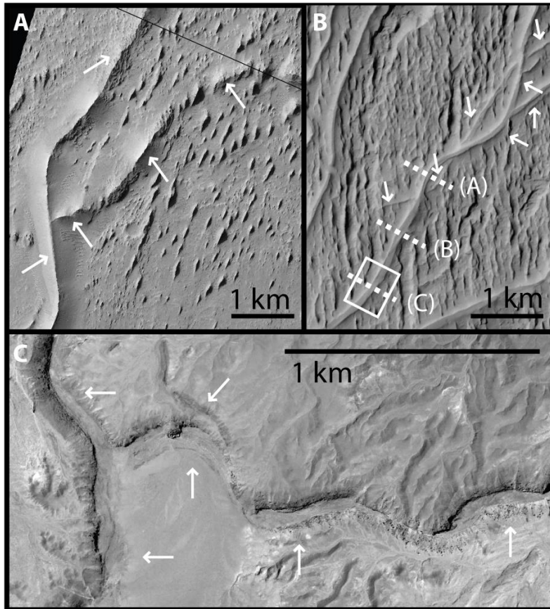
Fig. 1– Examples of sinuous ridges from Mars and Earth. Arrows point to ridges. A) Long ridge with a single branch in Aeolis Dorsa, Mars. Small parallel bumps are yardangs (Coordinates - 4.67, 151.13; HiRISE image PSP_010533_1755; credit: NASA/JPL/University of Arizona). B) At least two sets of stratigraphically distinct ridges on Mars with superposed yardangs. This is part of a larger ridge network that has been interpreted both as convergent flow to the lower left based on channel inversion and divergent flow to the upper right on the basis of deposit inversion (Lefort et al., 2012; 2015; DiBiase et al., 2013). White box indicates section shown in Fig. 15A, dotted lines denote cross section locations in Fig. 15B. (Coordinates -6.105, 151.479; Aeolis Dorsa, Mars; CTX image B18_016691_1740_XN_06S208W; credit: NASA/JPL/Malin Space
