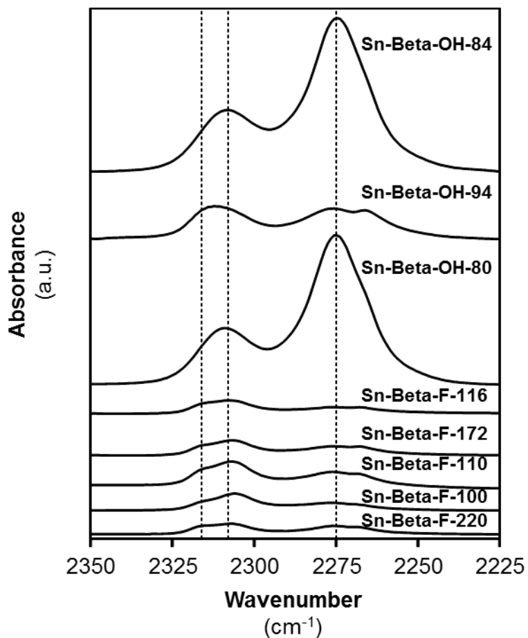
Figure S.5. IR spectra collected on \text{CD}_3\text{CN} -saturated Sn-Beta samples studied in this work. Spectra were normalized by combination and overtone modes for Si-O—Si stretches prior to the subtraction of spectra collected before \text{CD}_3\text{CN} adsorption. Dashed lines are drawn at 2308\text{ cm}^{-1} ( \text{CD}_3\text{CN} bound to closed Sn), 2316\text{ cm}^{-1} ( \text{CD}_3\text{CN} bound to open Sn), and 2275\text{ cm}^{-1} ( \text{CD}_3\text{CN} bound to silanols).
