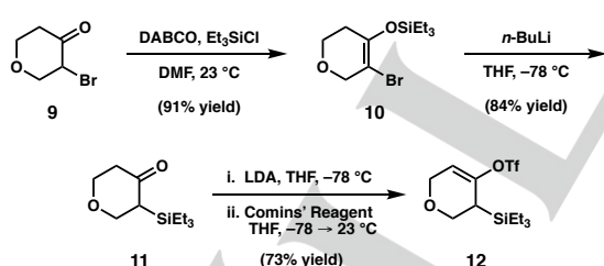
Scheme 1. Synthesis of silyl triflate 12 . DABCO=1,4-diazabicyclo[2.2.2]octane, DMF= N,N -dimethylformamide, THF=tetrahydrofuran, LDA=lithium diisopropylamide, Comins' Reagent= N -(5-Chloro-2-pyridyl)bis(trifluoromethanesulfonimide).
