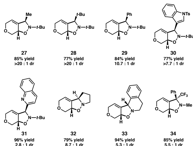
Figure 3. (3+2) cycloadditions with nitrones. The major diastereomeric product is shown. Yields reflect an average of two isolation experiments. Diastereomeric ratios were determined by ^1\text{H} NMR analysis of the crude reaction mixture. OTf=trifluoromethanesulfonate, Ts = para -toluenesulfonyl.
