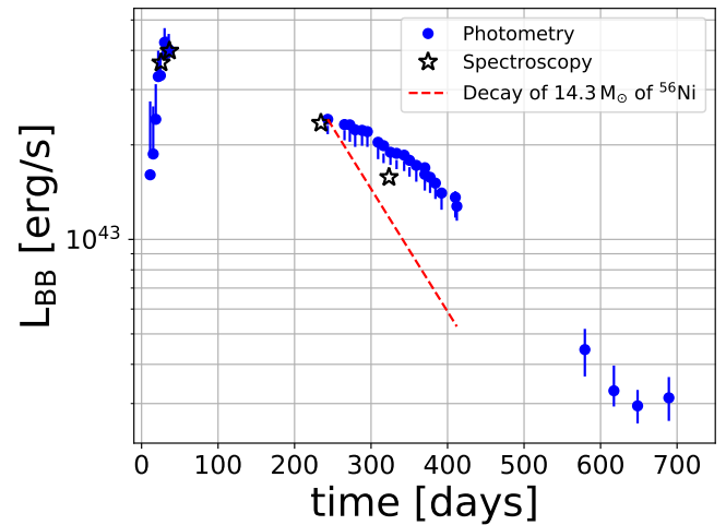
FIG. 7.— The evolution in time of the bolometric luminosity of a blackbody with the same radiation as PTF 12glz. The stars indicate the fits to the spectroscopic data. The dashed line shows the variation in luminosity caused by 14.3 M_{\odot} of ^{56}\text{Ni} radioactively decaying to ^{56}\text{Co} and then to ^{56}\text{Fe} . L_{BB} decays \approx 2 times slower, which suggests that radioactive decay is not sufficient to explain the decay of the light curve and that interaction or other sources of radiation play a role.
