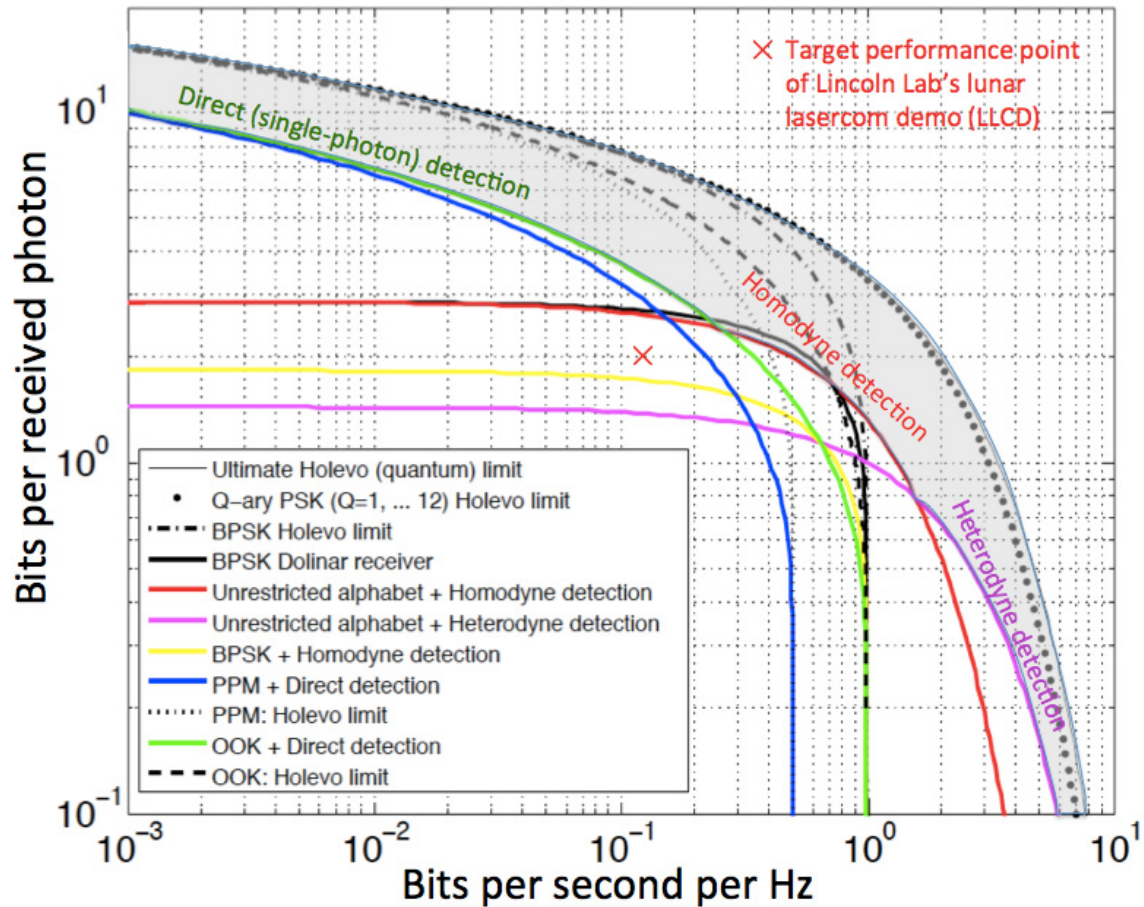
Figure IV-18 Photon versus spectral efficiency of a far-field optical channel. The colored (non-black) lines show the best performance achievable with standard techniques. The shaded area is the gap between achievable rate and the Holevo capacity.
