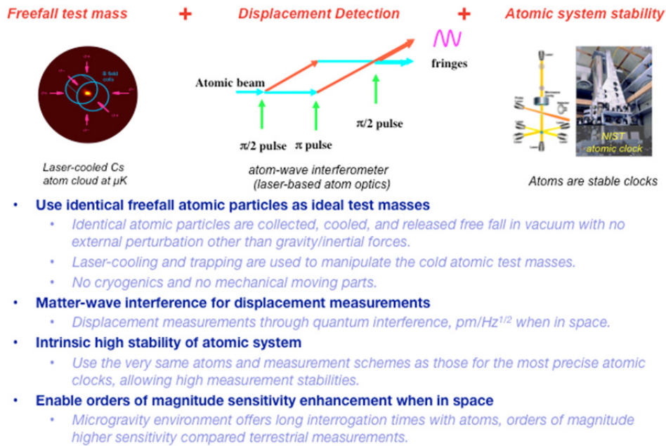
Figure IV-5 Unique aspects of atom interferometer based inertial sensors and their characteristics.
