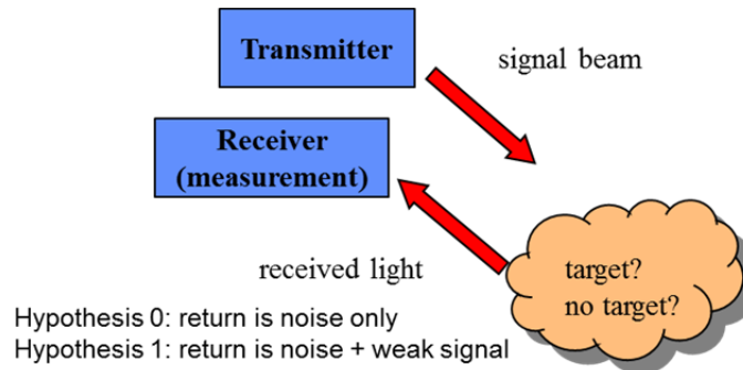
Figure IV-8 Quantum illumination concept for target detection in the presence of a weak signal return and high background.
