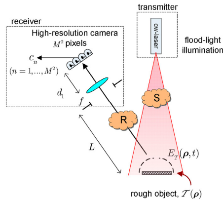
Figure IV-11 Block diagram of conventional floodlight LADAR. Cloud icons indicate atmospheric turbulence.
