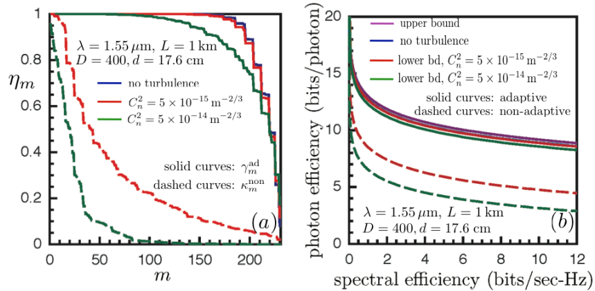
Figure IV-21 (a) LG/HG mode transmissivity results for a near-field link, (b) Ergodic Holevo capacity bounds: PIE vs. spectral efficiency.
