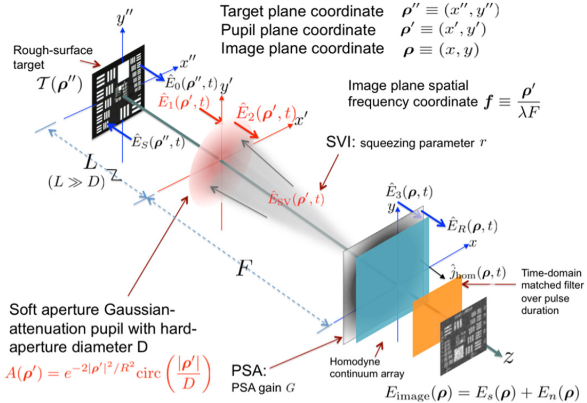
Figure IV-6 Notional configuration for Type-II laser radar receiver using squeezed-vacuum injection (SVI), phase-sensitive amplification (PSA), and homodyne detection to achieve improved angle resolution in a coherent-state, soft-aperture laser radar.
