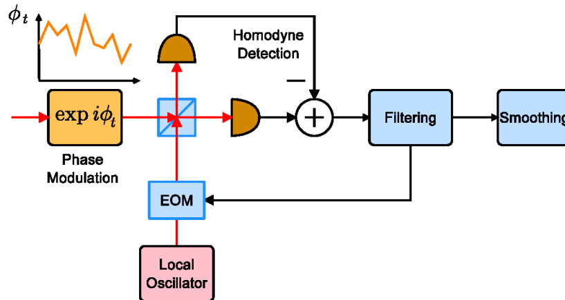
Figure IV-7 Schematic of a homodyne optical phase-locked loop for phase tracking and estimation.
