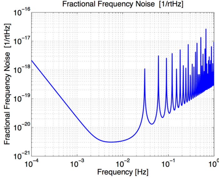
Figure IV-3 Fractional frequency stability of the separation between two LISA-like spacecraft.
