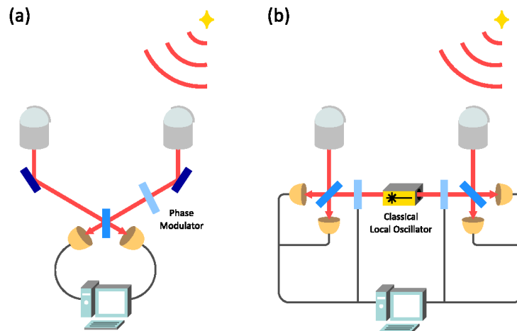
Figure IV-12 Schematics of (a) the direct detection scheme, an example of nonlocal quantum measurement, and (b) a local measurement scheme, which performs spatially separate measurements and permits only classical communication and control between the two sites. Examples of the latter include heterodyne and homodyne detection. Quantum theory shows that the nonlocal measurements are fundamentally much more accurate than any local measurement technique in stellar interferometry when the collected photon flux is low [Tsang2011b].
