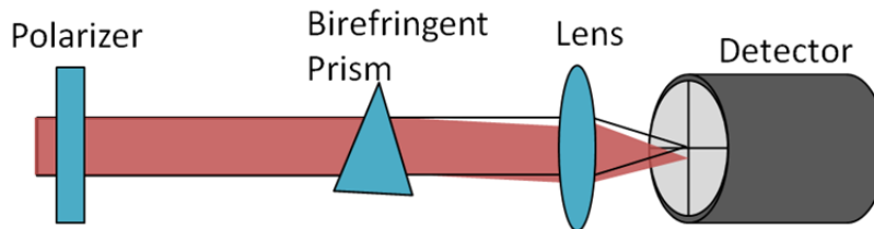
Figure IV-13 A standard technique to measure beam deflection is shown. A prism deflects the incident beam. The beam is focused onto a position sensitive detector, such as a quad-cell detector.
