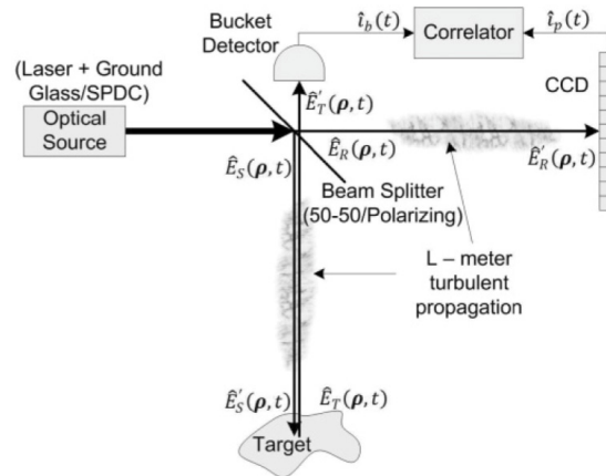
Figure IV-9 Block diagram for active ghost imaging for standoff sensing with either a quantum source or a classical source.
