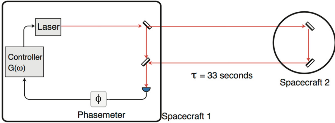
Figure IV-4 Schematic of locking the laser frequency to the arm length.
