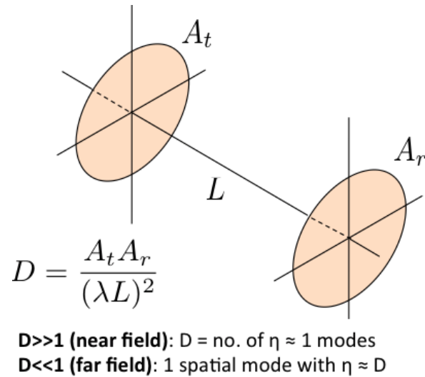
Figure IV-20 A line-of-sight free-space optical channel.
