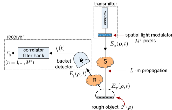
Figure IV-10 Computational ghost imaging block diagram for standoff sensing.
