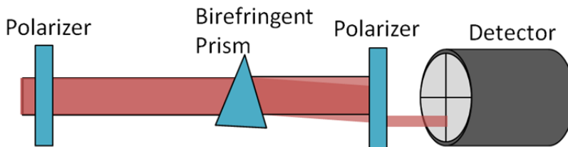
Figure IV-14 A weak value technique to measure beam deflection is shown. A beam with a pre-selected polarization is deflected by a prism. The beam is then post-selected on a nearly orthogonal polarization and sent to a position sensitive detector, such as a quad-cell detector.
