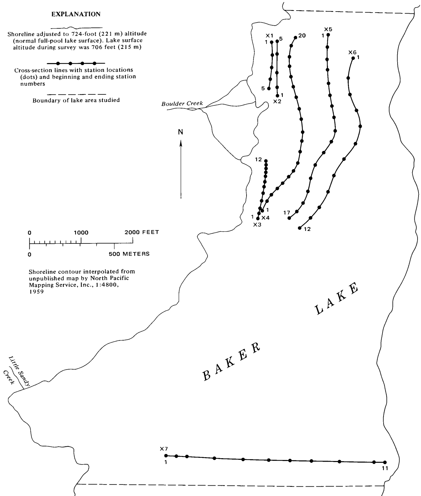
FIGURE 5.—Sketch of central Baker Lake showing cross-section and station locations for survey of September 3 and 4, 1975.
