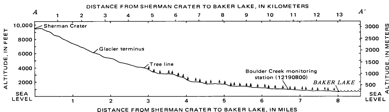
FIGURE 2.—Generalized profile along Boulder Creek valley (line of profile, A-A', shown in fig. 1).
