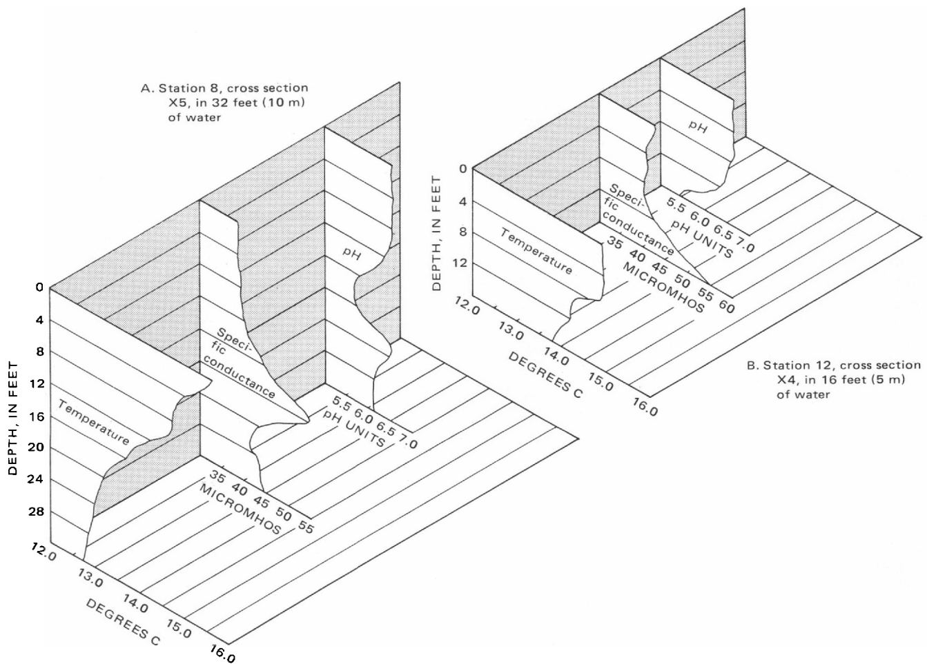
FIGURE 7.—Vertical profiles of temperature, specific conductance, and pH at two locations on Baker Lake (locations shown in fig. 5).
