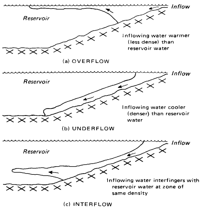
FIGURE 6.—Schematic sections showing overflow, underflow, and interflow in a reservoir from incoming stream water.
