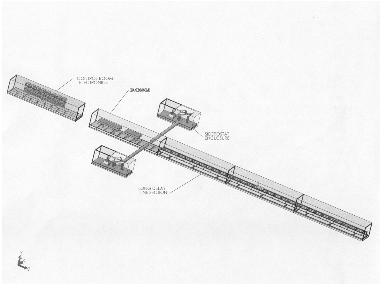
Fig. 1. A concept design for the API phase 1 instrument. The instrument would be modularized in shipping containers (represented as rectangular sections in the drawing above). The containers would be moved by overland traverse, as part of regular Concordia station cargo, to the Concordia base at Dome C. Once on site, the containers would be positioned and attached. All interferometer optics and electronics equipment would be mounted on damped, isolation mounts for shipping. Once the containers were attached, the isolation mounts would be removed and precision assemblies would mount to hard points. This approach allows the entire interferometer to be deployed and tested on sky in the Northern hemisphere prior to deployment to the Antarctic plateau. The instrument is designed to be upgraded with the addition of larger telescopes (2-meter-class) at the positions of the siderostats. In addition, the design accommodates additional delay range by adding additional long-delay line segments.
