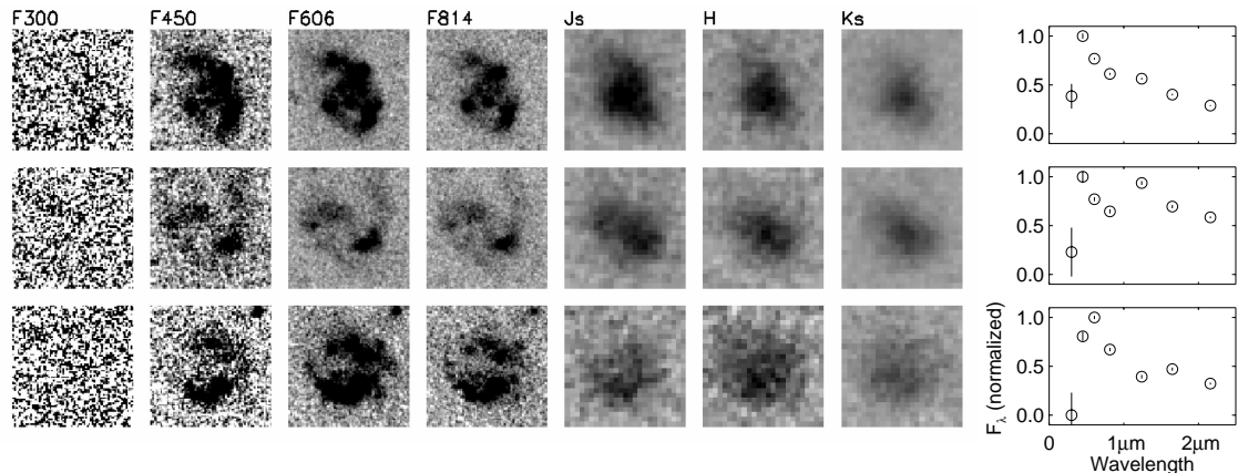
Figure 1. Morphology of the most extended U-drop galaxies in the HDF-S. The left panels show the WFPC2 U, B, V, I data, and right hand panels show our VLT/ISAAC J_s, H, K_s data. The images are 3 x 3 arcsec on a side. The intensity is proportional to F_\lambda , with arbitrary normalization for each galaxy. The right hand column shows the spectral energy distributions. As can be seen, these U-drop galaxies are large in extent, and can show prominent Balmer breaks. The K -band infrared images (rest-frame optical) are generally more centrally concentrated than the WFPC2 images; this is a physical change and not caused by the difference in image quality. The galaxy in the bottom row is spectroscopically confirmed at z_{spec} = 2.8 .
