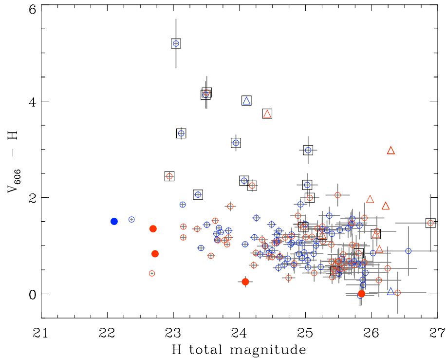
Figure 3. V_{606} - H versus H color-magnitude diagram (on the AB system) for galaxies in the K_s -selected catalog of the HDF-S that are photometrically at 1.95 < z_{phot} < 3.5 . Filled symbols indicate galaxies with spectroscopy, and the data points are grouped into two redshift ranges: 1.95 \leq z < 2.7 (red) and 2.7 \leq z < 3.5 . The number of candidates for red, evolved galaxies is much higher than in the HDF-N, as shown in a identical plot in Fig. 1 in Ref. 7 : we find 7 galaxies redder than V_{606,AB} - H_{AB} > 3 and brighter than H_{AB} < 25 , compared to one in the HDF-N. For easy comparison, we give the magnitudes and colors in the AB system, where V_{606,AB} = V_{606} + 0.12 and H_{AB} = H + 1.38 . Galaxies with S/N < 2 for the V_{606} measurement (triangles) are plotted at the 2\sigma confidence limit in V_{606} , indicating a lower limit on the V_{606} - H color. The subsample of galaxies having red J_s - K_s > 2.3 colors (open squares) are also indicated.
