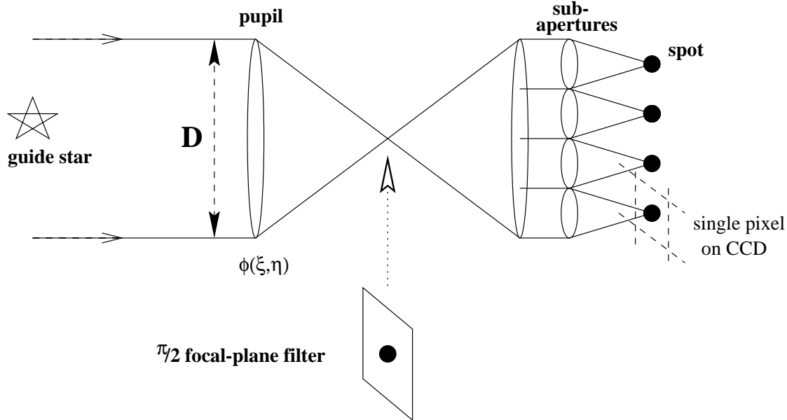
Figure 4. Schematic of the phase-contrast wavefront sensor. A focal-plane filter is inserted into the intermediate focal plane, as with the knife-edge WFS, but the filter in this case is transmitting, so no light is lost. The filter has an additional optical thickness of \pi/2 , and has a transverse size roughly matching the diffraction-limited spot size. In the reimaged pupil, subaperture spots have intensity directly proportional to the pupil phase in that subaperture, and may thus be measured by a single CCD pixel (see text).
