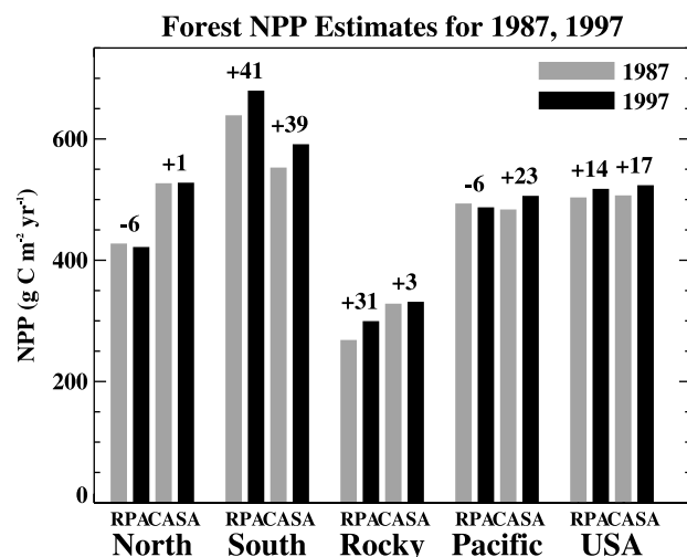
Figure 3. Regional estimates of NPP ( \text{g C m}^{-2} \text{yr}^{-1} ) from Resource Planning Act/Forest Inventory and Assessment (RPA/FIA) tree surveys and CASA for 1987 (gray bars) and 1997 (black bars). Numbers above the bars indicate the change from 1987 to 1997. For the RPA/FIA NPP values, dates for 1987 correspond to surveys in the 1970s and 1980s, and for 1997 to surveys in the 1990s and 1980s. For CASA, only forest biomes are used in the calculation, and 1987 represents the mean from 1982–1987 and 1997 the mean from 1988–1997. The Pacific region does not include Alaska or Hawaii.
