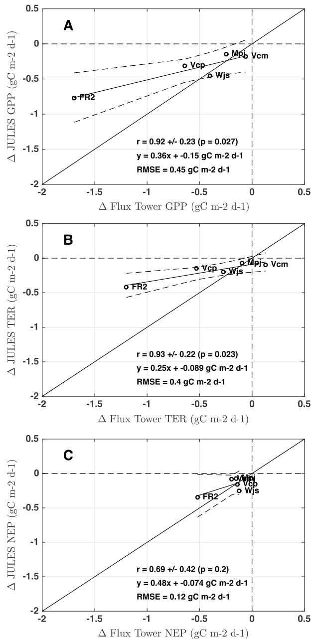
Figure 7. Regressions of annual CO 2 flux anomalies (difference of 2011 from 5+ year average) of JULES onto flux tower anomalies for (a) gross primary production (GPP), (b) terrestrial ecosystem respiration (TER), and (c) net ecosystem production (NEP). Model GPP is sampled at the same time as flux towers and in the grid cell closest to the tower location. Correlation ( r ), p value ( p ), slope/ y intercept ( y ), and root-mean-square error are also shown.
