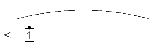
FIG. 2: An accelerated atom excites as an Unruh–DeWitt detector [5, 15], thereby emitting Unruh–Wald radiation.
