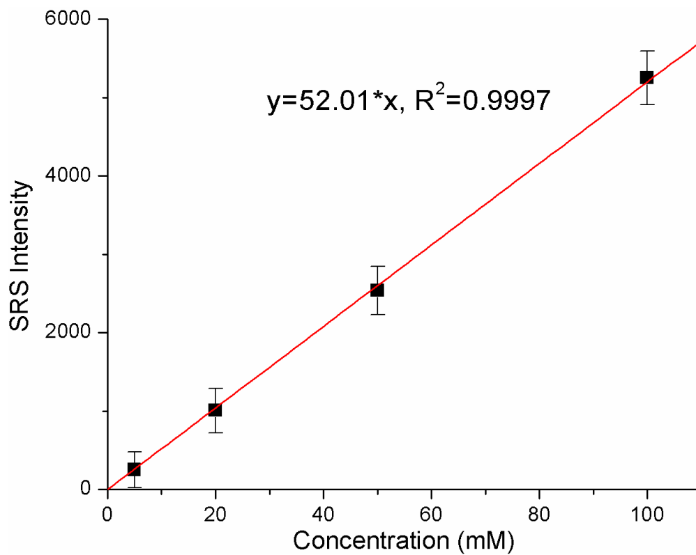
Figure S2. Correlation curve of SRS intensity at 2188\text{ cm}^{-1} with \text{D}_9 -choline PBS solution at different concentrations.
