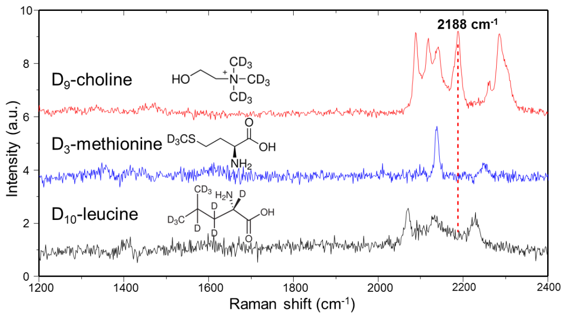
Figure S1. 2188 cm -1 as a characteristic Raman peak for D 9 -choline. Methyl C-D vibrational frequency is sensitive to local environment as shown in the comparison between D 9 -choline, D 3 -methionine and D 10 -leucine.
