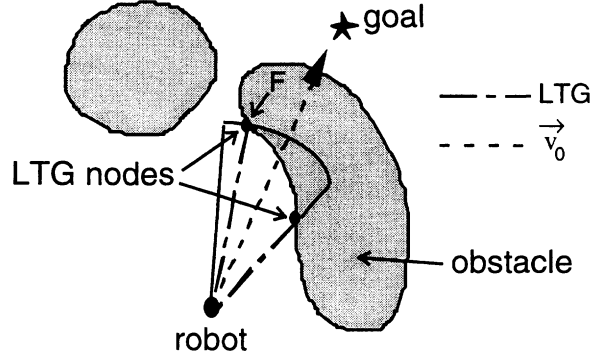
Figure 4. LTG calculated within W(x, \vec{v}_0) .
