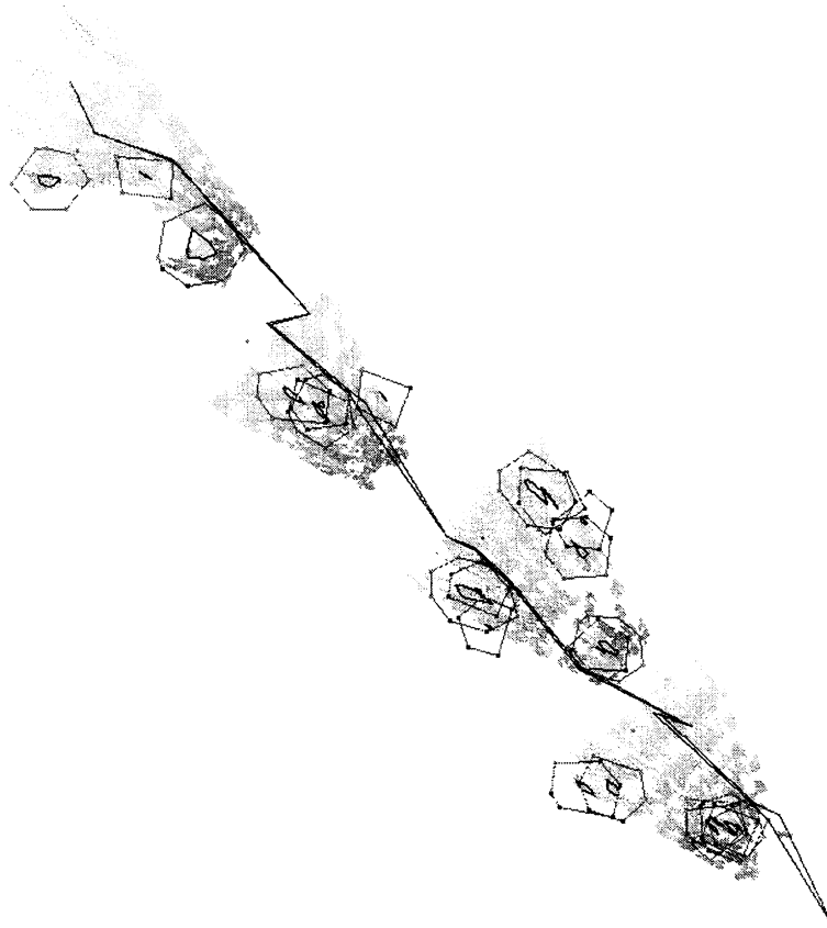
Figure 8. Results from a multi-step run in the JPL MarsYard. The path begins in the lower right corner of the image, toward a goal approx. 21 m distant in the upper left. Each wedge depicts a rangemap produced from mast imagery, and extends roughly 5 m from the imaging position. The obstacles are marked by a black convex hull, and a grey silhouette. Each subpath ends with an apparent “jag” in the path; these are not in fact motions, but rather the result of the localisation procedure run at the conclusion of each step. The second line echoing the path is the rover’s telemetry for the run.
