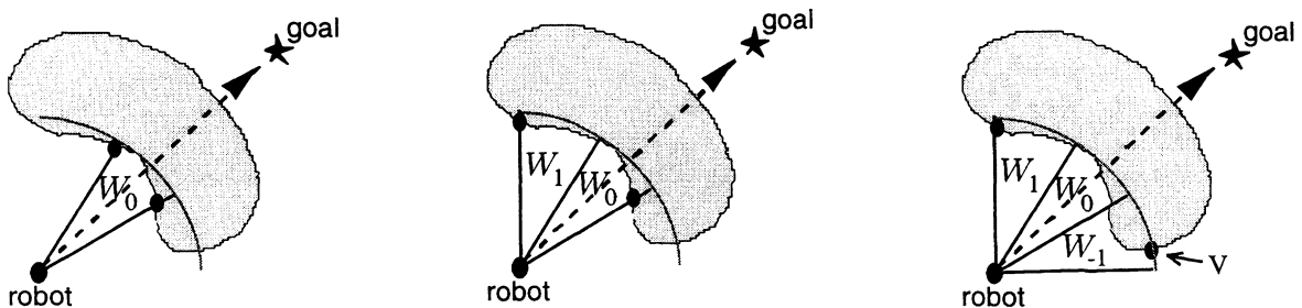
Figure 6. “Virtual BF .” The figure on the left depicts the first part of a “virtual BF ” step. The nodes of LTG(W_0) are marked with black circles. Since \nexists V \in \text{int}(LTG(W_0)) , the robot scans W_1 (center). Again, \nexists V \in \text{int}(LTG(W_0 \cup W_1)) , so the robot scans W_{-1} (right). Now, V \in \text{int}(W_0 \cup W_1 \cup W_{-1}) , so “virtual BF ” ends.
