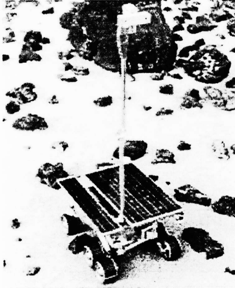
Figure 7. The Rocky7 Prototype Microrover, developed at JPL to test technologies for future missions. It is pictured here in the JPL MarsYard, an outdoor testing arena featuring simulated martian terrain.
