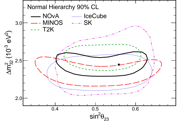
FIG. 11. Comparison of measured 90% confidence level contours for \Delta m_{32}^2 vs. \sin^2 \theta_{23} for this result (black line; best-fit value, black point), T2K [7] (green dashed), MINOS [6] (red dashed), IceCube [57] (blue dotted), and Super-Kamiokande [58] (purple dash-dotted).
