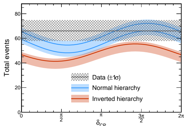
FIG. 9. Total number of \nu_e CC candidate events observed in the FD (gray) compared to the prediction (color) as a function of \delta_{\text{CP}} . The color lines correspond to the best fit values of \sin^2 \theta_{23} and \Delta m_{32}^2 from Table VII, with the upper two curves (blue) representing two octants in the normal mass hierarchy ( \Delta m_{32}^2 > 0 ) and the lower curve (red) the inverted hierarchy ( \Delta m_{32}^2 < 0 ). The color bands correspond to 0.43 \leq \sin^2 \theta_{23} \leq 0.60 . All other parameters are held fixed at the best-fit values.
