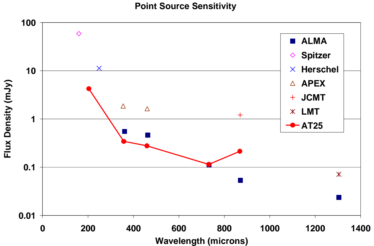
Figure 1: 5-sigma, 10,000 second point-source, continuum sensitivity of various current and planned sub-mm telescopes. Spitzer, Herschel, APEX, JCMT are confusion limited. The AT25 is confusion limited at 850 microns.
