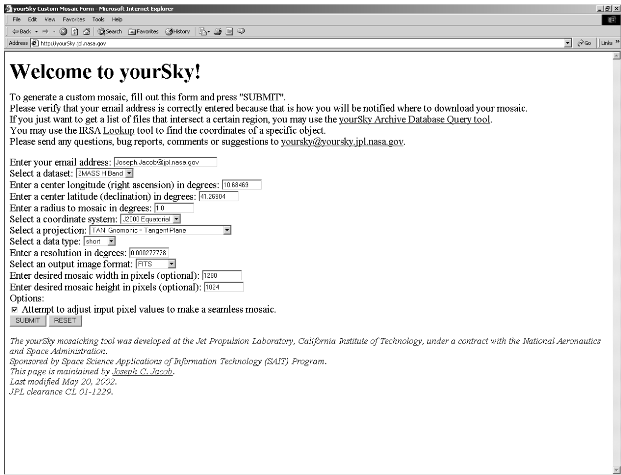
Figure 2. yourSky custom mosaic form interface.
