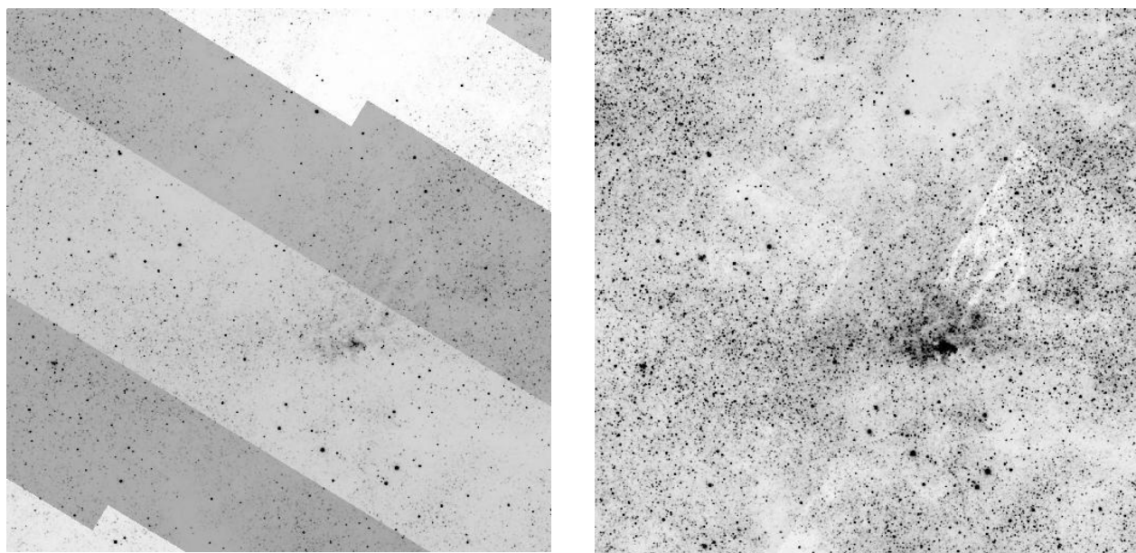
Figure 5. 2MASS H band center of the galaxy mosaic constructed from 16 2MASS image plates at 1 arc second resolution without (left) and with (right) background matching.
