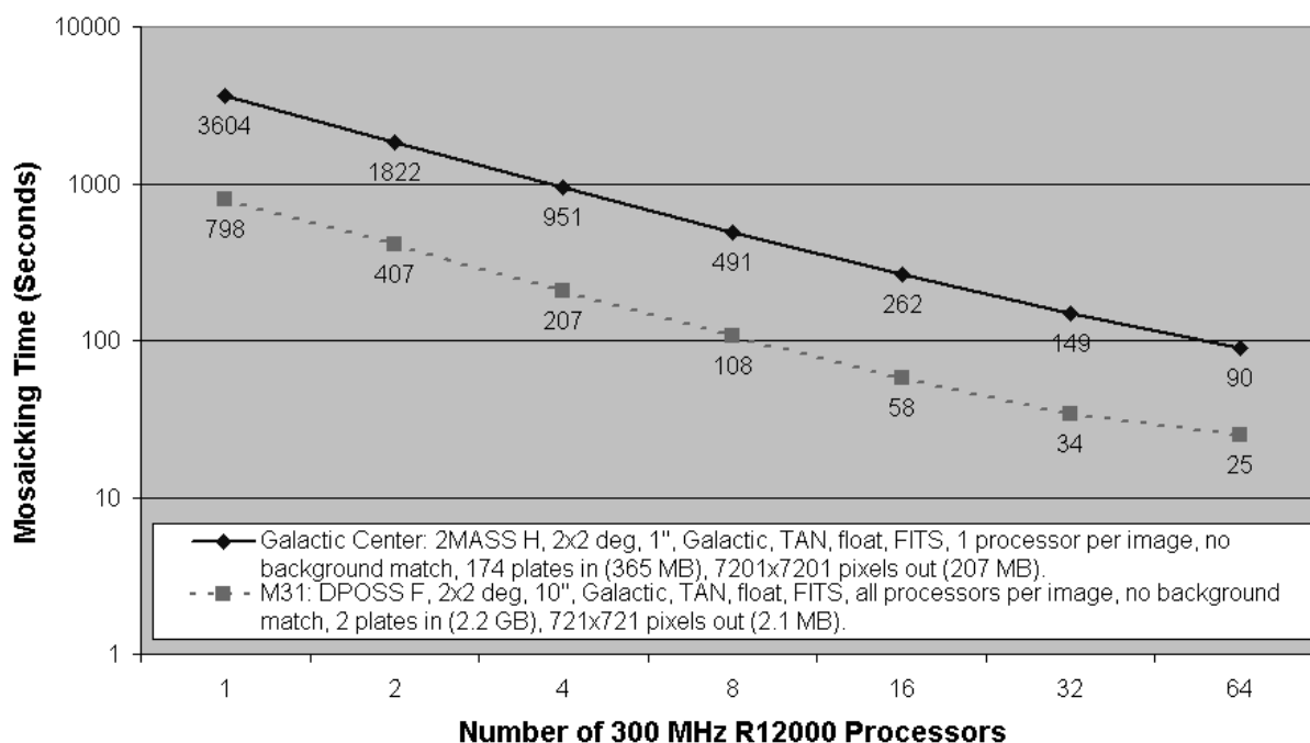
Figure 7. Mosaicking software performance on an SGI Origin 2000 for two different mosaic parameters, a 2x2 degree 1 arc second resolution mosaic of the galactic center in 2MASS with one processor assigned to each input image plate and a 2x2 degree 10 arc second resolution mosaic of M31 in DPOSS with all processors assigned to each input image plate.
