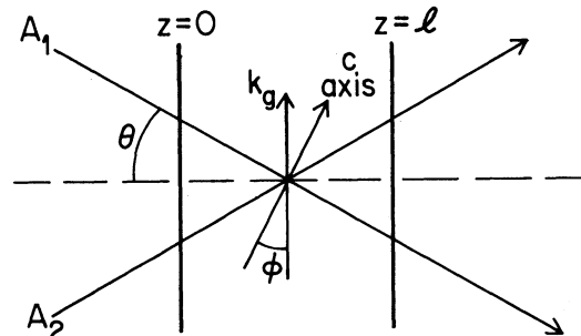
Figure 1. Two beam coupling geometry
