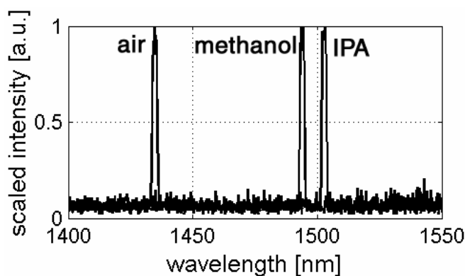
Figure 3. Measured laser spectra of photonic nanolaser sensor when filled with air, methanol and IPA
