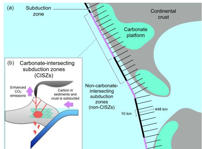
Figure 1. (a) Schematic representation of the \sim 450 km long cross-profile “whiskers” that are constructed along subduction zones (purple and black), spaced 10 km apart in the direction of subduction. The carbonate polygons (light blue) of the carbonate platform mask have a value of 1 (including those on the continental and oceanic crust), and elsewhere the grid values are zero. All whiskers that intersect, at some point along their length, with the carbonate platforms in the mask will contribute 10 km to the total count of carbonate-intersecting subduction zones. (b) Schematic representations of carbonate-intersecting continental subduction zones. Carbonate platforms become buried over time, forming reservoirs in the crust. Through assimilation and decarbonation reactions, arc magmas interact with upper-crustal carbonates and liberate significantly more \text{CO}_2 emissions than at non-intersecting continental arcs.
