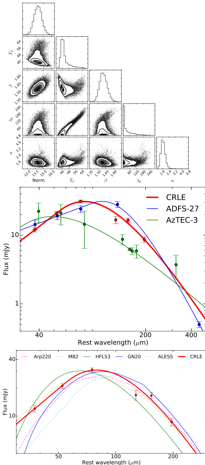
Figure 5. Modified blackbody (MBB) fits to the FIR SED in CRLE. Top: Corner plot of the model parameter posterior distribution. Middle: FIR SED comparison to other z > 5 DSGFs (AzTEC-3 and ADFS-27; Riechers et al. 2014a, 2017). CRLE shows peak emission at intermediate rest-wavelengths between the hot, compact starburst AzTEC-3 and the early-stage merger ADFS-27. Bottom: Comparison to other low and high redshift FIR SED templates (Silva et al. 1998; Riechers et al. 2013; Magdis et al. 2011; Swinbank et al. 2014).
