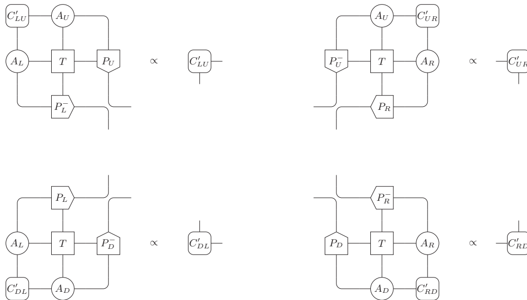
FIG. 1. Fixed point equations for the CTMs.
