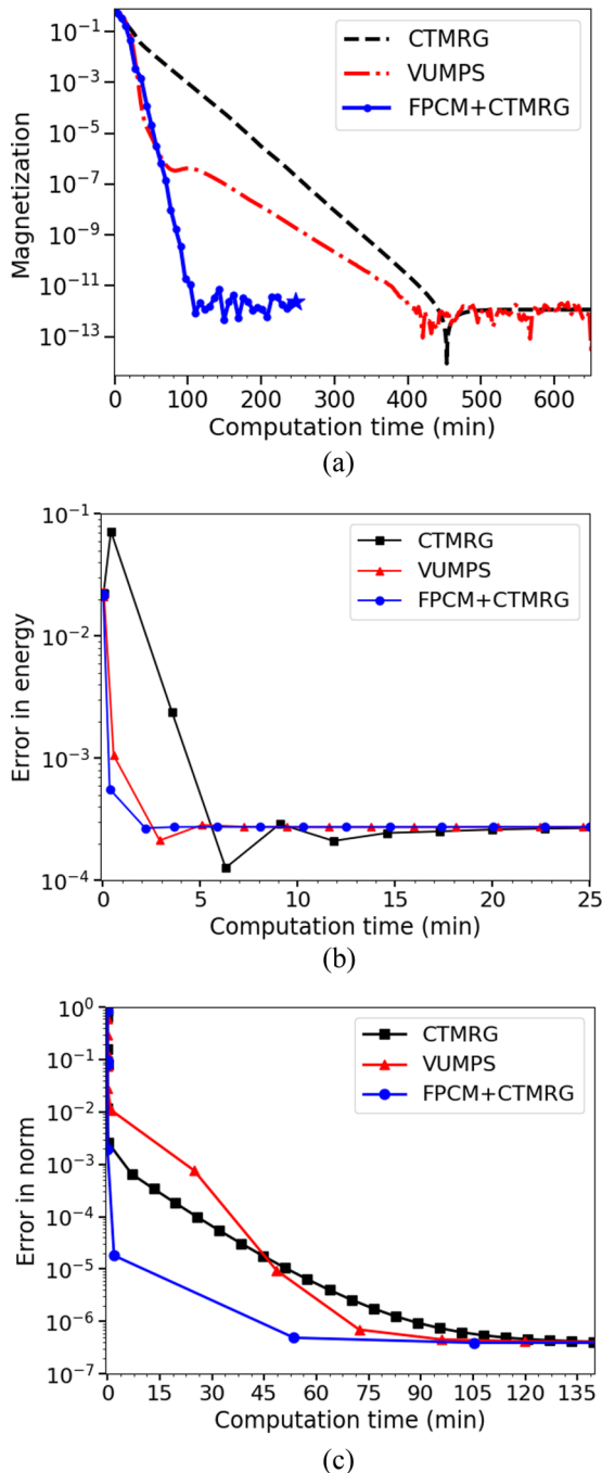
FIG. 4. (a) Plot of magnetization for the 2D classical XY model, for network bond dimension d = 25 and boundary MPS bond dimension \chi = 50 . (b) Plot of error in energy (compared to Monte Carlo results) for the 2D quantum Heisenberg model. The network bond dimension is d = 25 (or PEPS bond dimension D = \sqrt{d} = 5 ), and the MPS boundary bond dimension \chi = 100 . (c) Plot of error in the norm (where the “exact” results is taken to be an extrapolation of the norm in the limit of a large environment bond dimension) of the chiral RVB PEPS. The network bond dimension is d = 9 (or PEPS bond dimension D = \sqrt{d} = 3 ), and the boundary MPS bond dimension is \chi = 800 .
