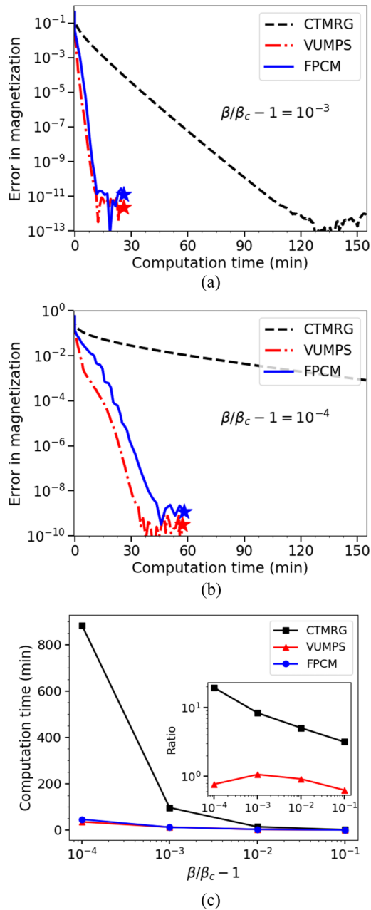
FIG. 2. Plots (a) and (b) show the error in the magnetization for the isotropic 2D classical Ising model as a function of computation time at two temperatures near criticality, where (b) is closer to criticality than (a). The network has a bond dimension of d = 2 , and a boundary MPS bond dimension of \chi = 600 is used. A fully symmetric CTM ansatz is used for CTMRG and the FPCM, and full symmetry is exploited in VUMPS. The speedup of VUMPS and the corner method over CTMRG increases as one gets closer to criticality. Stars indicate the environment tensors have reached a fixed point, and data points beyond those points are numerical fluctuations and were not shown in order to simplify the plot. Plot (c) shows convergence time as a function of inverse temperature above criticality, \beta/\beta_c - 1 , for the 2D classical Ising model. For all data points, a boundary MPS bond dimension of \chi = 600 is used. All data is converged to an error in the magnetization of < 2 \times 10^{-9} . The inset shows the ratio of the convergence time of CTMRG and VUMPS with respect to the FPCM convergence time (note the logarithmic scale).
