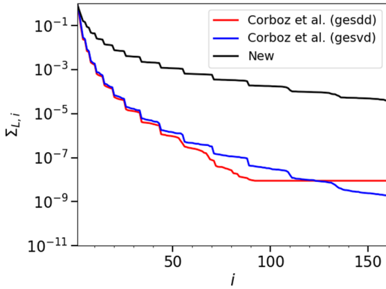
FIG. 5. Comparison of spectra that need to be inverted to perform the biorthogonalization in different versions of the asymmetric CTMRG algorithm. Note that what is plotted, \Sigma_{L,i} , are the square roots of the singular values that are calculated during the biorthogonalization. See the main text for details.
