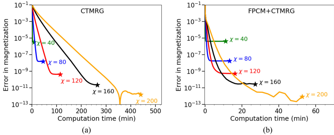
FIG. 3. Plots of error in magnetization for the isotropic ferromagnetic 2D classical Ising model at \beta/\beta_c - 1 = 10^{-3} with random nonunitary gauge transformations introduced on the horizontal and vertical links, as shown in Eq. (43). This artificially breaks the lattice symmetry in order to test each method on an asymmetric network. Plot (a) shows results for the asymmetric CTMRG algorithm by Corboz et al. in Ref. [51] and plot (b) shows results for the FPCM introduced in this work combined with the CTMRG algorithm used in (a).
