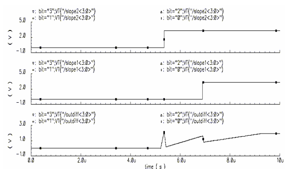
Figure 15. Simulated waveforms for the CDS with a full scale input. The transitions in the bottom waveform correspond to range shifting to progressively less sensitive ranges and are recorded in the top two digital traces. The analog signal is digitized at the last time marker on the right.
