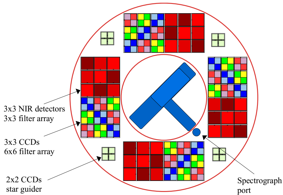
Figure 6. The SNAP focal plane working design. The two axis symmetry of the imager filters allows any 90^\circ rotation to scan a fixed strip of the sky and measure all objects in all nine filter types. The central rectangle and solid circle are the spectrograph body and its light access port, respectively. The spectrum of a supernova is taken by placing the star in the spectrograph port by steering the satellite. The four small, isolated squares are the star guider CCDs. The inner and outer radii are 129 and 284 mm, respectively.
