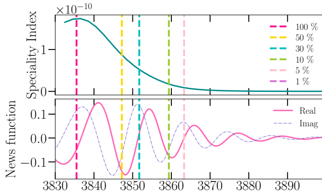
FIG. 14: This figure is similar to Fig. 13 but for Specialty Index. We plot this separately as it is an independent measure and decays rapidly compared to the other measures. Further, we do not indicate the 1% of peak line because of numerical noise (cf. Fig. 9) which leads to unreliable root finding for time of percentage decrease.
