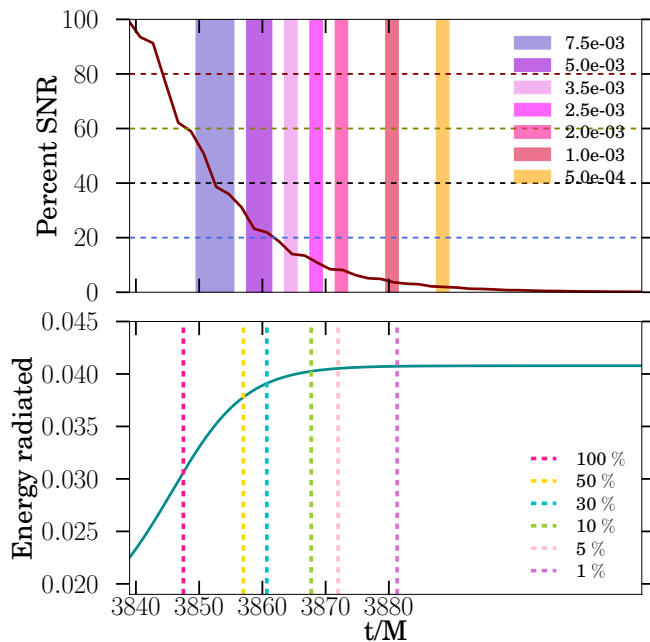
FIG. 20: The top panel of this figure shows the percentage decrease of SNR from the peak value. The % SNR is set to 100 at t_{\text{merger}} . For this plot, we evaluate Eq. (28) with varying lower bounds for the integration. The dashed horizontal lines correspond to \{80, 60, 40, 20\} % SNR. On the same plot, we mark the perturbation amplitude bands for a direct comparison between perturbation amplitude and statistical error. Notice that by the time the perturbation amplitude near the BH decreases by an order of magnitude, there is only a few percent of SNR left in the signal, emphasizing the sharp trade-off between the systematic biases arising from modeling the post-merger as perturbed Kerr and the statistical uncertainty arising due to exponential decay of signal amplitude. The bottom panel shows the total energy radiated in units of M during the merger-ringdown. This is calculated by integrating Eq. (30). Again, we have plotted the concomital percentage decrease of the Kerrness measures from their peak values for an easy comparison between the statistical and systematic errors associated with the choice of the start time of ringdown. In particular, the constant settling in the total radiated energy occurs between the time when the Kerrness measures have decayed to 5 – 1% of their peak values, implying that at these times the GW is very weak in amplitude.
