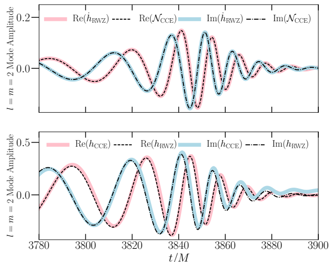
FIG. 19: Comparison between the strain h calculated using CCE and RWZ methods. All waveforms are presented in terms of the l = m = 2 mode. We use the fact that the strain is the integral of the news function to cross-check the methods. The top panel shows the CCE news function \mathcal{N}_{\text{CCE}} compared to \dot{h}_{\text{RWZ}} , the derivative of the RWZ strain. The bottom panel shows h_{\text{CCE}} , the integral of the CCE news function, compared to the RWZ strain h_{\text{RWZ}} . We find good agreement until late times, when h_{\text{CCE}} begins to drift due to the numerical integration scheme (Simpson's rule).
