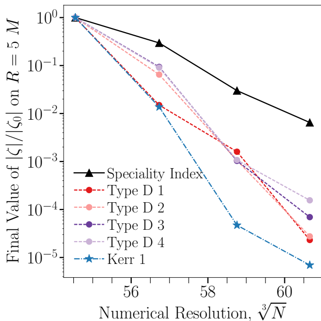
FIG. 12: Exponential convergence of the noise floor of each Kerrness measure on the final timestep of the BBH simulation. Each measure \zeta is presented as an average over a 2-sphere of R = 5M (where the measures have settled to a noise floor), normalized by |\zeta_0| , the average of the lowest resolution. The resolution is indicated by \sqrt[3]{N} , where N is the number of spectral collocation points. The convergence to zero shows that the noise floor observed in Fig. 9 is a numerical noise floor, rather than real a physical artifact. We have also testing this convergence behavior on a 2-sphere R = 5M and verified that the behavior is consistent (although more noisy).
