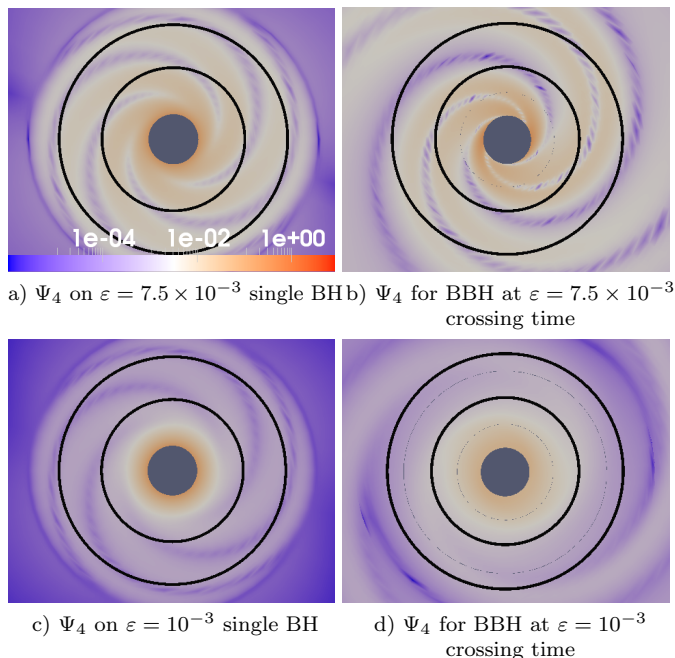
FIG. 16: \Psi_4 in the equatorial plane for both a single BH with an l = m = 2 perturbation of amplitude \varepsilon = 7.5 \times 10^{-3} and \varepsilon = 10^{-3} ( left panel ), and for the BBH ringdown ( right panel ) at times that achieve the same Kernness as ( left panel ). For all cases, Kernness is matched on a coordinate 2-sphere of R = 5M . The two black circles correspond to coordinate radii R = 5M and R = 8M . The Gaussian envelope of width R = 8M , as described in Fig. 4, can be seen in the plots for the single BH cases. Notice that although the two systems look similar, allowing us to infer the BBH simulation perturbation amplitude, the mapping does have some imperfections.
