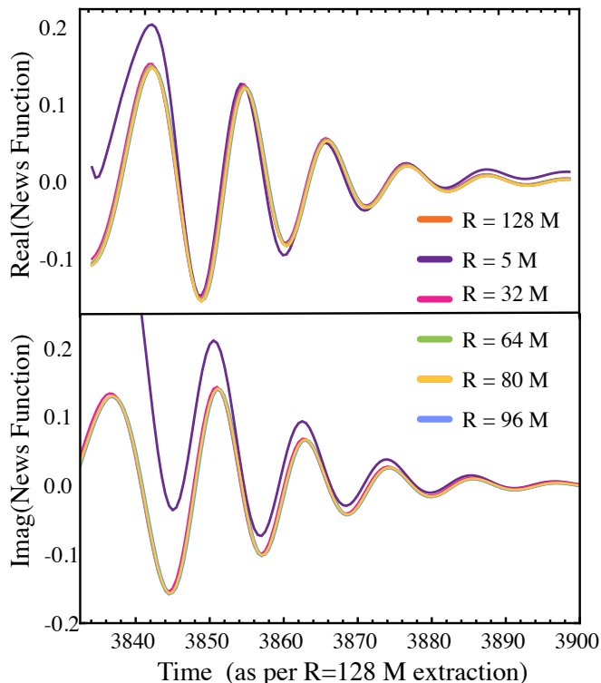
FIG. 6: The l = m = 2 mode of the news function seen at \mathcal{S}^+ extracted from worldtube boundaries of R = 5 M , 32 M , 64 M , 80 M , 96 M and 128 M . The horizontal axis corresponds to the time stamps associated with the news function corresponding to CCE from R = 128 M . The top panel shows the real part and the bottom panel shows the imaginary part of the news function. The alignment of news functions has been done such that the overlap is maximized. The transformation that changes the gauge from a non-inertial to an inertial observer has not been applied to any of the extractions. All of the extractions beginning with R = 32 M seem to agree with one another. Notice that the amplitude of the news function extracted from R = 5 M deviates from the other extractions, especially in the first cycle. Nevertheless, the phase evolution between the news function from extraction radii seem to agree.
