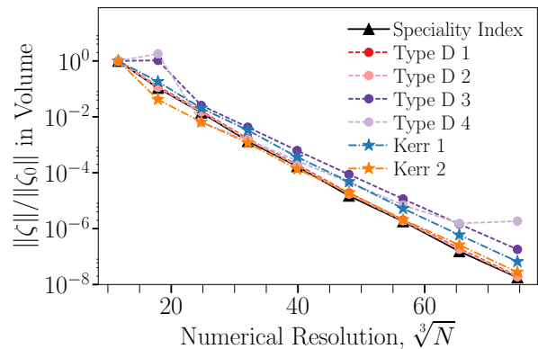
FIG. 5: Convergence of Kerrness measures on a numerical BH in Kerr-Schild coordinates with dimensionless spin \chi = (0.2, 0.3, 0.4) . We observe exponential convergence towards the theoretical value of zero with numerical resolution. For each measure \zeta , we present \|\zeta\|/\|\zeta_0\| , the L2 norm over the spatial slice normalized by the L2 norm of the lowest resolution. The resolution is expressed \sqrt[3]{N} , where N is the number of spectral collocation points in the domain.
