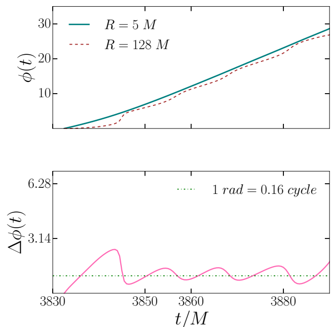
FIG. 7: The phase discrepancy between the news function extracted from a worldtube radius of R = 5 M and R = 128 M . The news functions are aligned to maximize the overlap. The top panel presents the phase evolution of the news function for each extraction radius. The bottom panel shows the fractional difference defined as \phi_{128} - \phi_5 . Notice that the phase difference is significant at the very beginning but quickly decreases to an acceptable level for our analysis. We notice that the phase difference oscillates about 1 radian, indicating the level of error we introduce by - a) not performing the final gauge transformation, b) imposing no-ingoing condition for CCE.
