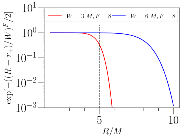
FIG. 4: Envelope function from Eq. (20), for various width and falloff parameters, \{W, F\} . We show how the envelope parameters affect an extraction radius of R = 5M (marked by the dashed black line). For our chosen values of \{W = 6M, F = 8\} , the envelope is at \sim 1 and R = 5M , while for \{W = 3M, F = 8\} , the envelope affects the perturbation amplitude at R = 5M . We have checked that using a smaller envelope does not change the qualitative behavior of our results.
