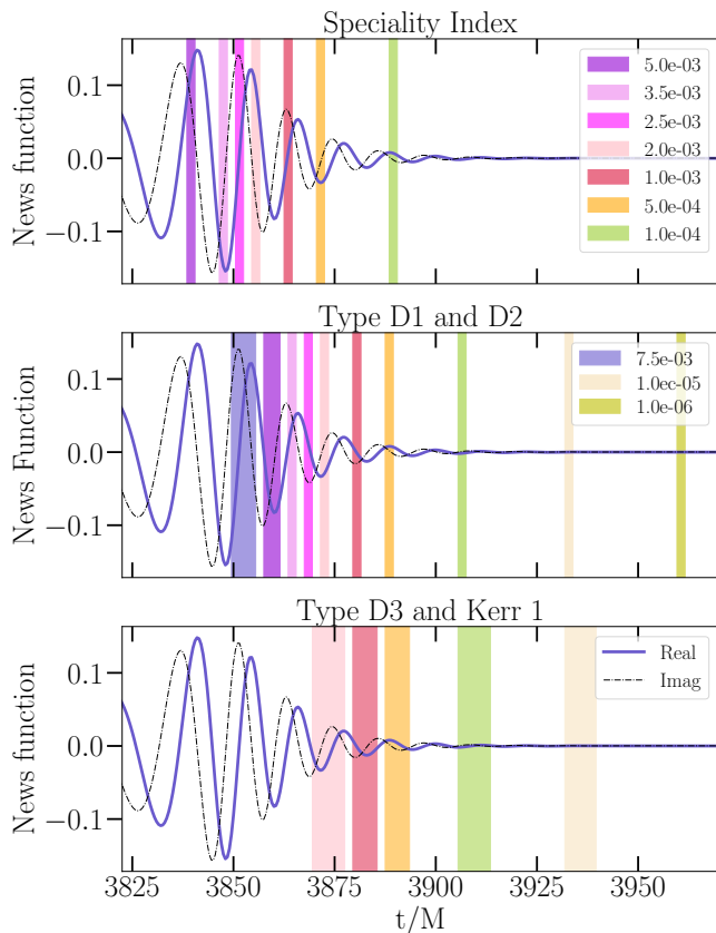
FIG. 18: Mapping the inferred perturbation amplitude close to the BH onto the news function. The top panel shows the spread in the crossing times computed using just the Specialty Index, the middle panel uses only the algebraic measures and the bottom panel utilizes only the geometric measures. Notice that amplitudes larger than 2 \times 10^{-3} do cross the post-merger timeslices when computed using the geometric measures and that the crossing time spreads in them are relatively large, suggesting a difference in the symmetry of a perturbed Kerr metric and the post-merger BBH spacetime. However, this does not seem to be reflected when we just consider the algebraic measures as they have a relatively small spread in the crossing time. The spread in the crossing time of the Specialty Index is equal to the sampling rate.
