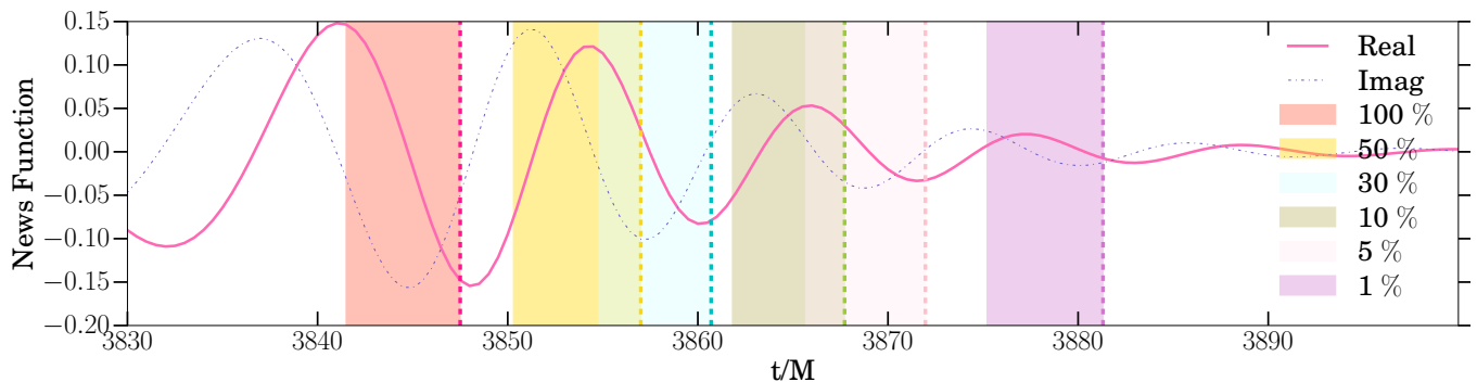
FIG. 15: The concomitant decrease of all of our Kernness measures. The dashed lines indicate the time at which all the measures decay to at least the indicated % of peak. The bands color the region in which different measures decrease to the indicated % of peak. Notice that there is about half a cycle spread in each of these bands. Therefore, the dashed lines provide a conservative idea of the validity of the choice of the start time for data analysis. We have specifically included the spread of these bands as a quantifier of error bounds in the statements of validity made further in this paper. Furthermore, one could shrink the right boundary of these shaded bands if one combines the Kernness measures with appropriate weights based on their sensitivity to the spacetime curvature and the final remnant’s effective potential.
