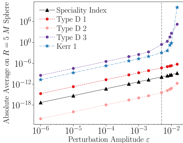
FIG. 3: Behavior of absolute Kerrness measures with perturbation amplitude \varepsilon . We compute this on an l = m = 2 QNM perturbed Kerr BH with the same mass and spin as the final remnant in the BBH simulation we consider in this paper. We average each measure on a coordinate 2-sphere of R = 5M . The behavior is initially quadratic with \varepsilon for all measures. At larger amplitudes \varepsilon \geq 5 \times 10^{-3} , Type D 2, D 3, D 4, and Kerr 1 show higher-power dependence, and hence non-linearity. We show this \varepsilon_{\text{crit}} \sim 5 \times 10^{-3} by a dashed vertical line. The lines between the points are only used to visually connect them (rather than being fits).
