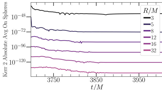
FIG. 11: Kerr 2 measure throughout the post-merger BBH simulation, averaged on a variety of coordinate 2-spheres of radius R . The values remain relatively constant and low, indicating that no NUT charge is gained during ringdown.
