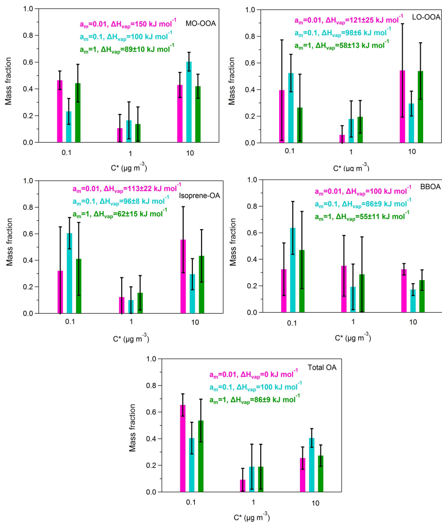
Figure A4. Predicted volatility distributions of the OA PMF factors and total OA. The error bars are estimated using the approach of Karnezi et al. (2014). The green bars represent the results for a_m = 1 (base case), the cyan bars correspond to the solution for a_m = 0.1 and the pink bars are the results for a_m = 0.01 .
