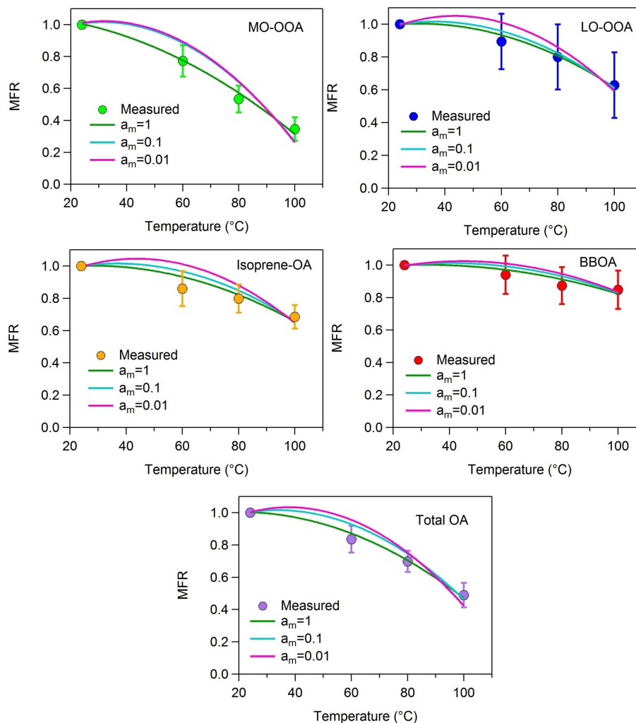
Figure A3. MFRs of the loss-corrected PMF OA factors and total OA. The circles denote the measurements with the 1 standard deviation of the mean, the green lines represent the best-predicted MFR for a_m = 1 (base case), the cyan lines correspond to the best-predicted MFR for a_m = 0.1 and the pink lines stand for the predicted MFR for a_m = 0.01 .
