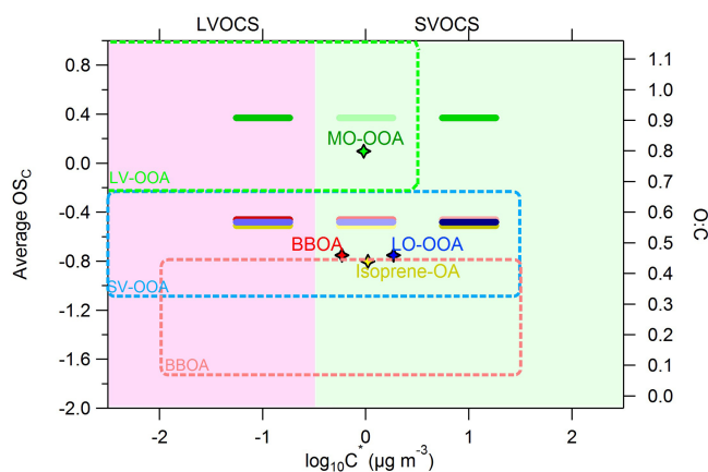
Figure 5. Average carbon oxidation state OS_C (left y axis) and O:C ratio (right axis) versus the saturation concentration in terms of \log_{10} C^* . The horizontal bars are the volatility distributions of the SOAS PMF factors: MO-OOA (green), LO-OOA (blue), isoprene-OA (yellow) and BBOA (red). The darker the color of the horizontal bars the higher the mass fractional contribution for the corresponding C^* bin. The diamonds represent the average \log_{10} C^* value for a given PMF factor. The green, light blue and pink dashed areas are the locations of the LV-OOA, SV-OOA and BBOA PMF factors as proposed by Donahue et al. (2012).
