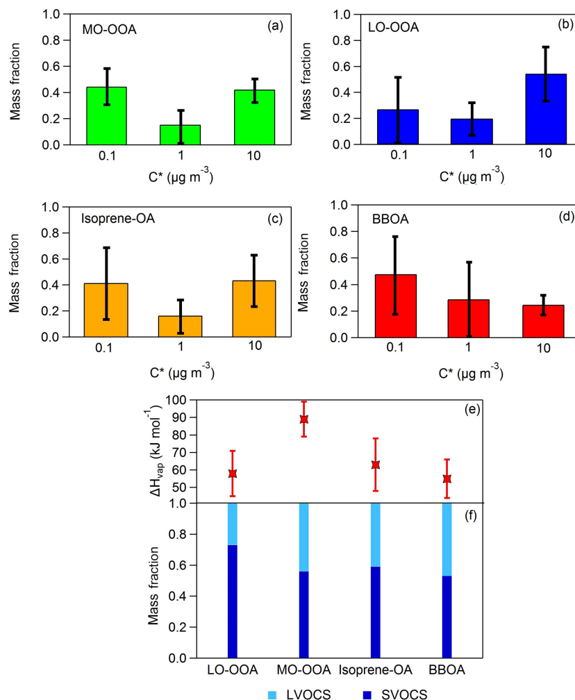
Figure 3. (a–d) Predicted volatility distributions of the OA PMF factors. The error bars correspond to the uncertainties derived using the approach of Karnezi et al. (2014), (e) vaporization enthalpies comparison between the four OA factors and (f) volatility compositions comparison between the four OA factors.
