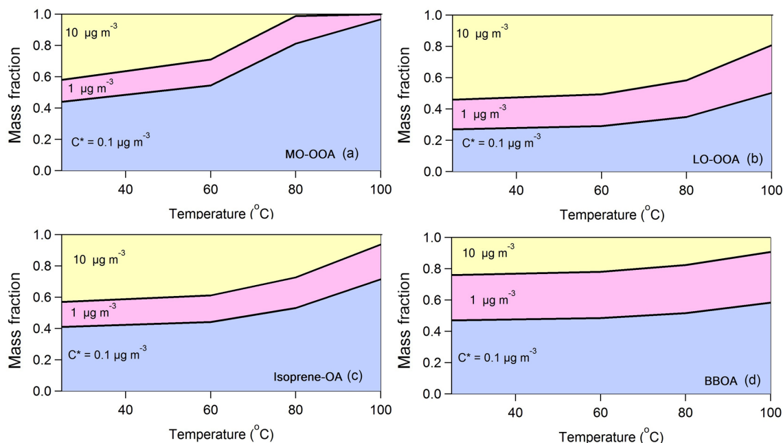
Figure 4. The predicted composition in terms of C^* for (a) MO-OOA, (b) LO-OOA, (c) isoprene-OA and (d) BBOA after passing through the thermodenuder as a function of the temperature. The model predicts, as expected, that the less volatile material with C^* = 0.1 \mu\text{g m}^{-3} dominates the composition of the remaining aerosol after the TD as the temperature increases for all factors. However, there are significant differences in the evolution of the composition of the various factors.
