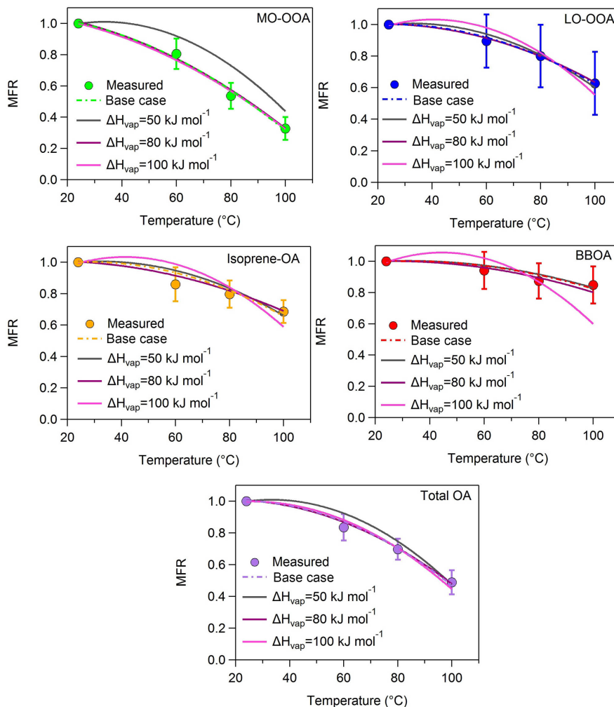
Figure A1. MFRs of the loss-corrected PMF OA factors and total OA for fixed values of the vaporization enthalpy. The circles denote the measurements with the 1 standard deviation of the mean, the dash lines correspond to the base case, the grey lines represent the case of a constant \Delta H_{\text{vap}} of 50 kJ mol -1 , the magenta lines stand for the case of a constant \Delta H_{\text{vap}} of 80 kJ mol -1 and the pink lines correspond to the case of a constant \Delta H_{\text{vap}} of 100 kJ mol -1 .
