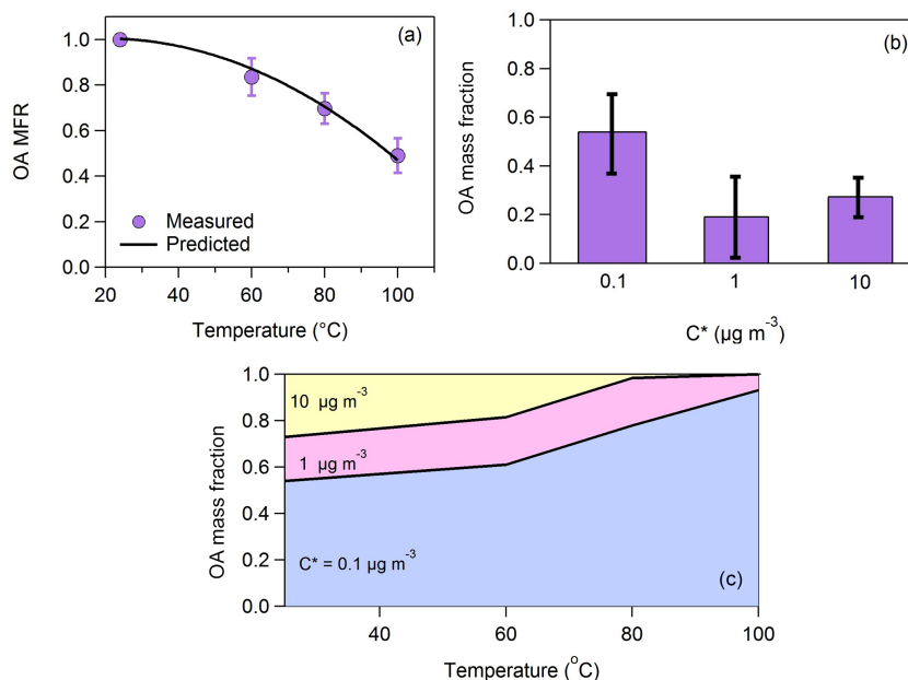
Figure 1. (a) Loss-corrected MFR of the total OA. The purple circles correspond to the measurements and the uncertainties to 1 standard deviation of the mean. It is assumed that \text{MFR} = 1 at T = 24 °C. The black line is the model fit estimated using the approach of Karnezi et al. (2014). (b) The total OA volatility distribution. The uncertainties have been estimated according to the algorithm of Karnezi et al. (2014). (c) The predicted volatility distribution after passing through the thermodenuder as a function of the temperature.
