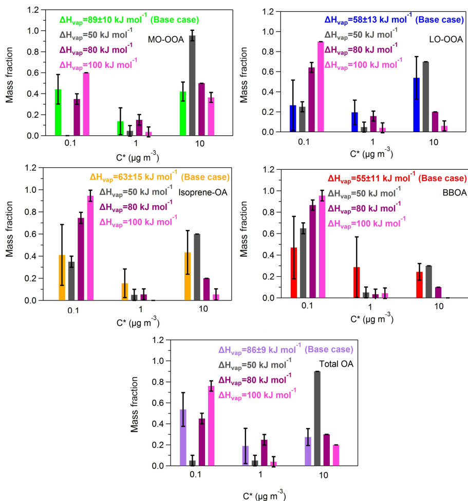
Figure A2. Predicted volatility distributions of the OA PMF factors and total OA for fixed vaporization enthalpy. The error bars are estimated using the approach of Karnezi et al. (2014). The grey bars represent the results of a constant \Delta H_{\text{vap}} of 50 \text{kJ mol}^{-1} , the magenta bars correspond to the solution of a constant \Delta H_{\text{vap}} of 80 \text{kJ mol}^{-1} and the pink bars are the results for the case of a constant \Delta H_{\text{vap}} of 100 \text{kJ mol}^{-1} . The green, blue, orange, red and purple bars stand for the base case solutions of MO-OOA, LO-OOA, isoprene-OA, BBOA and total OA.
