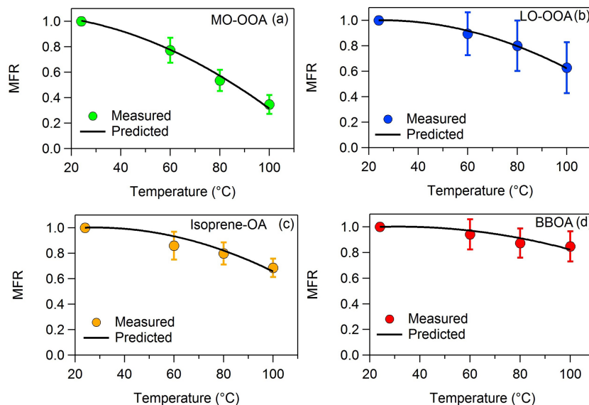
Figure 2. MFRs of the loss-corrected (a) MO-OOA, (b) LO-OOA, (c) isoprene-OA and (d) BBOA. The circles represent the measurements with the 1 standard deviation of the mean. The black line corresponds to the best-predicted MFR using the algorithm of Karnezi et al. (2014).
