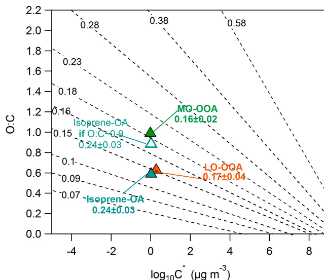
Figure 6. O : C ratios versus the average volatility as \log_{10}C^* . The black isolines correspond to the theoretically intrinsic \kappa suggested by Nakao (2017). The triangles denote the SOAS PMF factors. The hygroscopicity of the SOAS PMF factors has been transformed into the intrinsic \kappa , using the water solubility results of Xu et al. (2017). The open cyan triangle corresponds to the isoprene-OA with a hypothetical O : C = 0.9.
