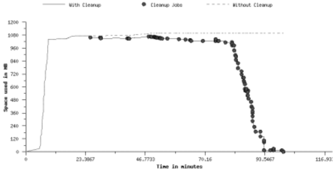
Fig. 9. Small LSC workflow data footprint over time with and without cleanup.
