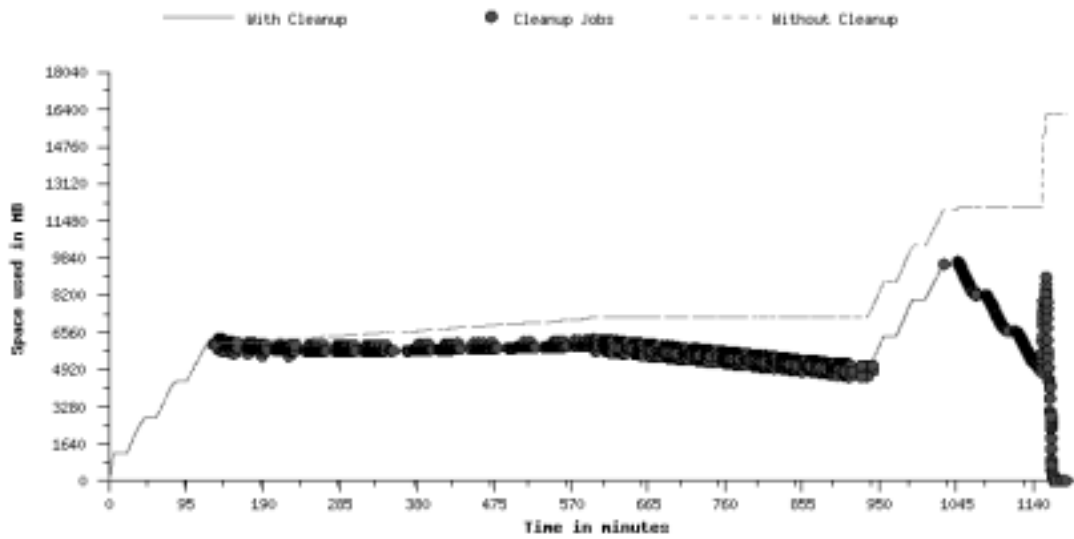
Fig. 8. Four degree square Montage workflow data footprint over time.
