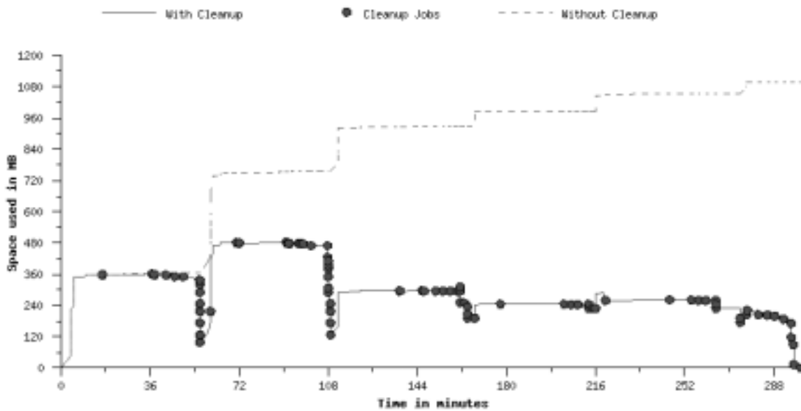
Fig. 20. Actual Grid behavior of the optimally restructured LSC workflow.
