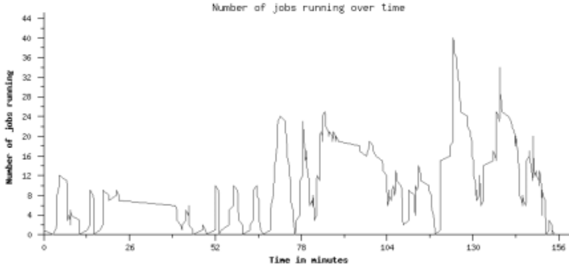
Fig. 22. Task execution profile of the moderately restructured LSC workflow.
