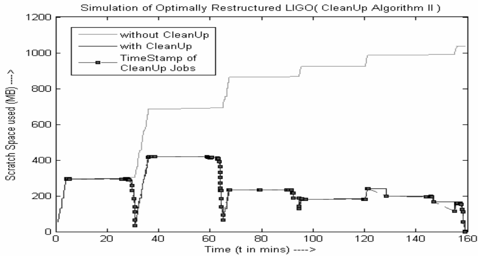
Fig. 19. Simulated behavior of the optimally restructured LSC workflow.
