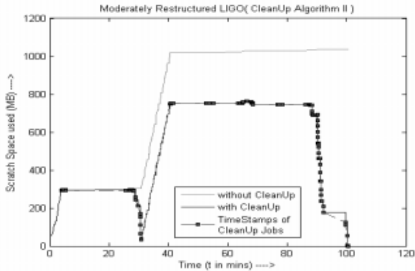
Fig. 15. Simulated behavior of the moderately-restructured workflow.
