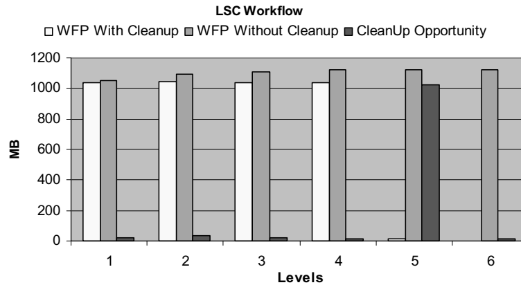
Fig. 10. The workup footprint (WFP) with and without cleanup and the cleanup opportunities at each level of the LSC workflow.
