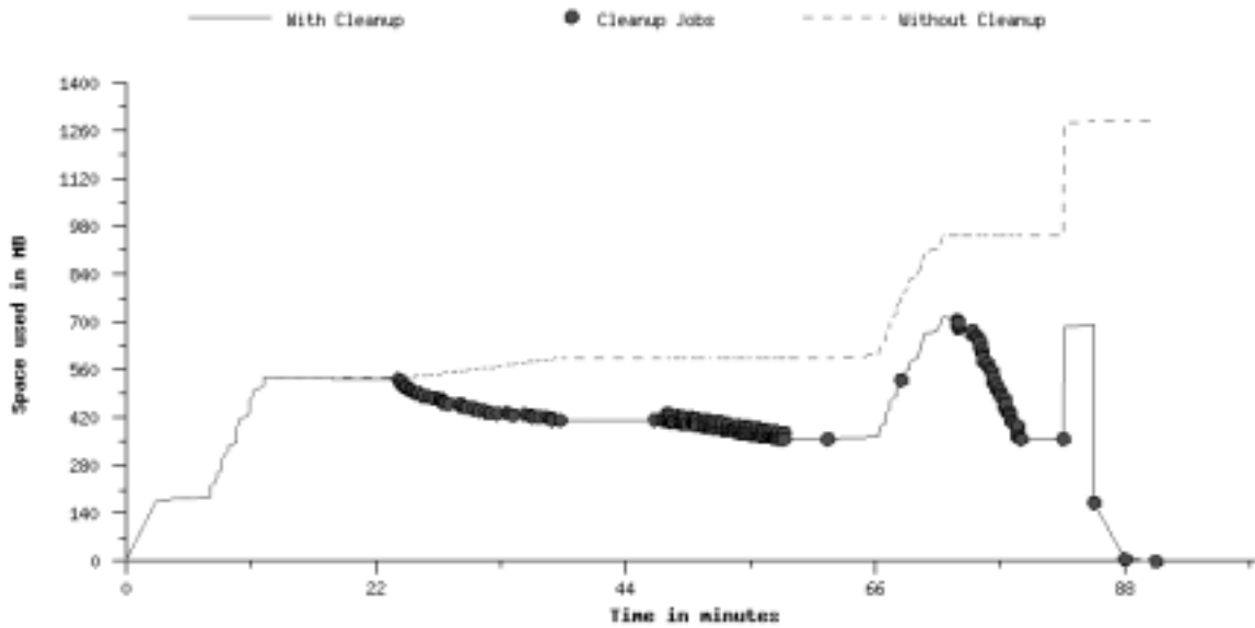
Fig. 6. One degree square Montage workflow data footprint over time.
