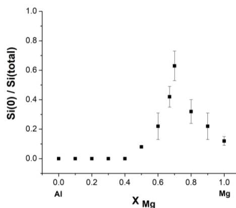
Figure 7. Formation of elemental Si (determined from XPS technique) as a function of Mg and Al composition.
