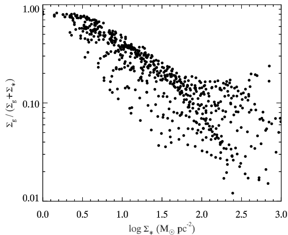
Figure 5. The distribution of \gamma = (1 + z_s/z_s)^{-1} as a function of \Sigma_* for all annuli in the sample from Leroy et al. (2008). This term determines the amount by which Eq. 5 should be multiplied by in order to obtain the true value of Q_{\text{thermal}}\tau .
