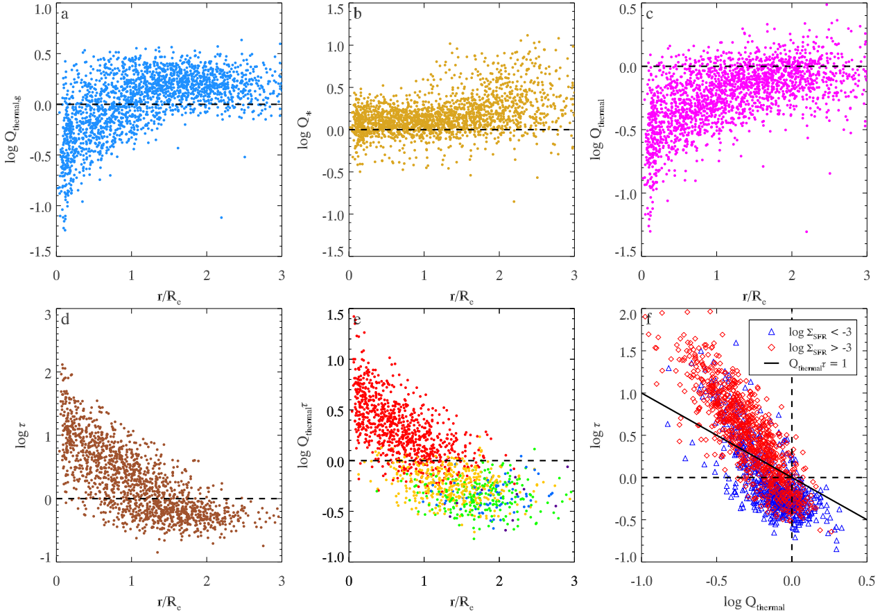
Figure 6. Properties of our MaNGA sample after approximating \Sigma_g based on the data in Fig. 5 and incorporating the stellar component. Panels (a)–(e) show the radial dependence of Q_{g,thermal} , Q_* , Q_{thermal} , \tau , and Q_{thermal}\tau . The color-coding in panel (e) is the same as that of Fig. 4a. Panel (f) shows the distribution of annuli in \tau, Q_{thermal} parameter space. This analysis supports our claim that disc will reach the threshold for disc stability before they reach the threshold for self-shielding.
