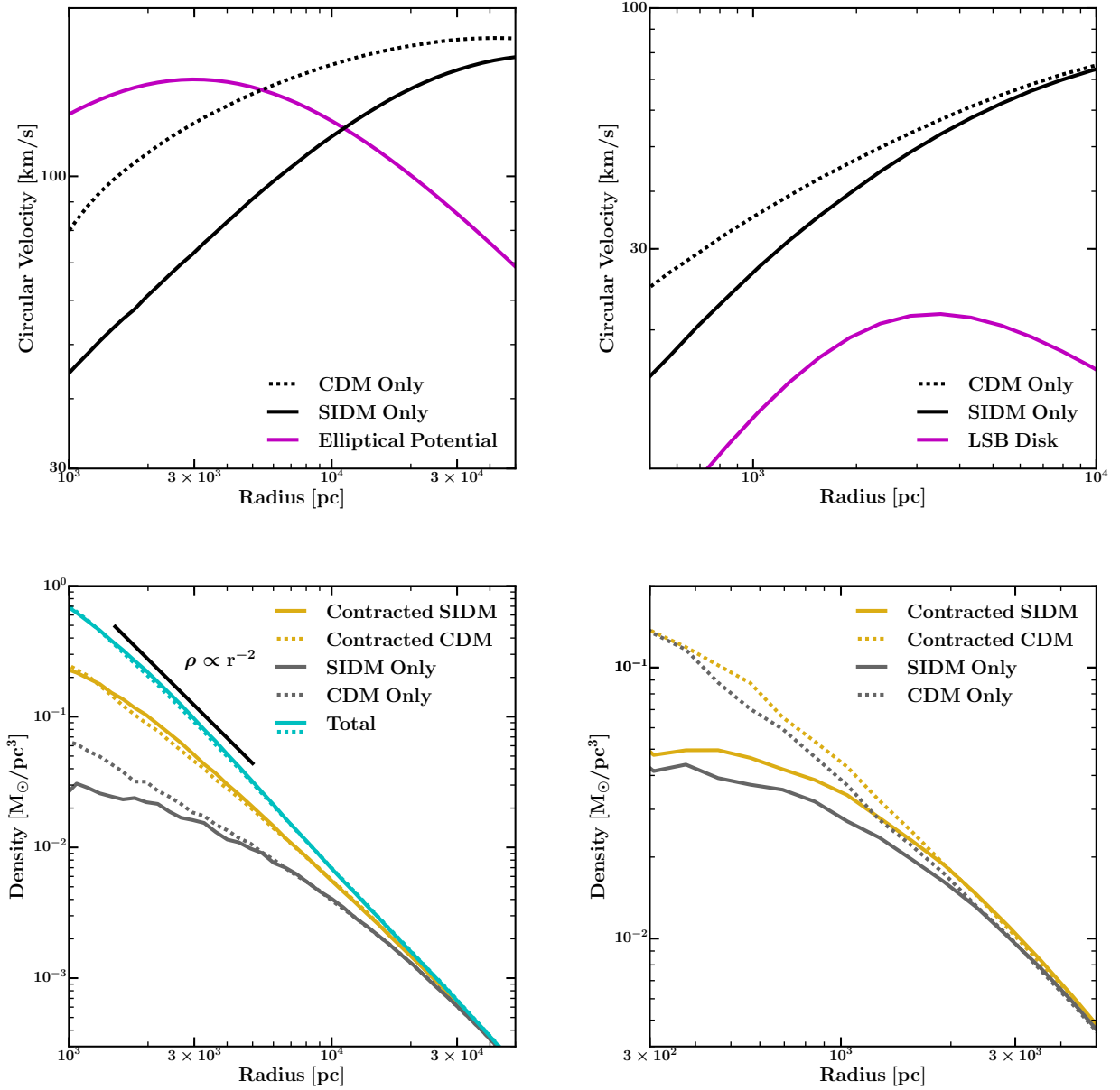
Figure 3. Initial rotation curves and final DM differential density profiles for our elliptical and LSB galaxy simulation simulated in both CDM and SIDM. Left: Elliptical Simulations. The top panel shows the rotation curves for our CDM and SIDM halos as well as for the added Hernquist potential, displaying how the halo becomes baryon-dominated within 5 kpc. The bottom panel shows the response of the halos to the added potential; as in the MW disk above, there is very little difference between the two contracted halos. We also include the total (DM plus galaxy potential) density profiles in cyan, and an r^{-2} power-law for comparison. Right: LSB simulations. The top panel shows the rotation curves for the initial CDM and SIDM halos along with the central disk potential, which contributes far less to the central mass and density of these halos. The lower panel shows that this relatively shallow baryonic potential has a much smaller impact on the host halo; there is very little difference between the initial and contracted CDM halos. The SIDM halo contracts slightly more, but still retains a core of lower density than the initial CDM halo.
