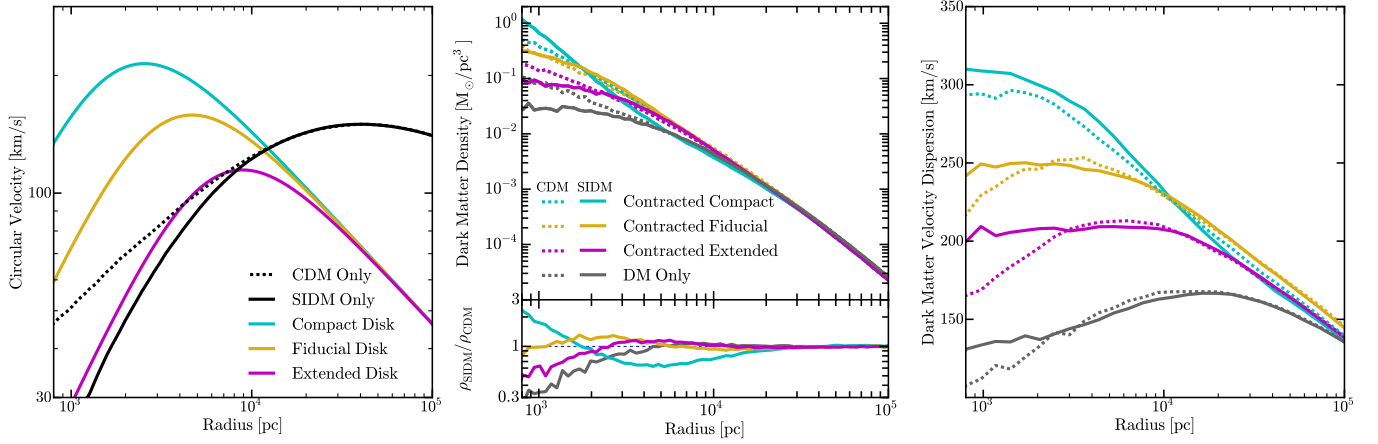
Figure 1. Left: The black lines show circular velocity profiles for dark-matter only Milky Way size halos (SIDM, solid; CDM, dashed). The colored lines show the circular velocity profiles of three imposed baryonic potentials: Fiducial Disk (yellow), Extended Disk (magenta), and Compact Disk (cyan). Middle: Dark matter density profiles without (grey) and with (colored) response to the grown disk potentials. The lower panel shows the ratio of the SIDM run to CDM run as a function of radius for each set of simulations. Right: Velocity dispersion profiles of the same halos, which demonstrate isothermal cores for the SIDM runs, as expected. Note that the relative effect of baryonic contraction is much more substantial in SIDM: the central densities at 600 pc increase by a factor of \sim 70 from the non-contracted case to the Compact Disk case in SIDM, compared to only a factor of \sim 5 in the CDM case. Interestingly, the Fiducial Disk runs in SIDM and CDM have very similar normalizations, though the SIDM simulation does show a small core developing within \sim 800 pc. The Compact Disk, on the other hand, has led to core-collapse in the SIDM halo, resulting in a much higher central density than even the contracted CDM halo. Core collapse is expected when the velocity dispersion has a negative gradient within the scattering radius, as is clearly the case for the Compact Disk in the right panel.
