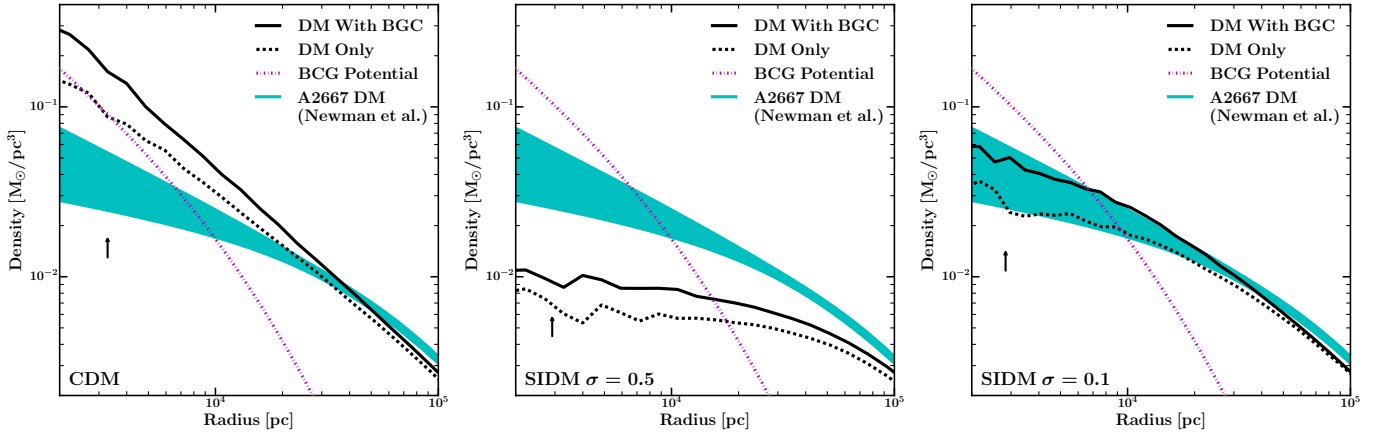
Figure 5. Density profiles for our simulations of cluster Abell 2667, along with the inferred dark matter density profile from Newman et al. (2013a). Even before contraction, our CDM halo (left) is too dense and the contracted SIDM profile with \sigma/m = 0.5 \text{ cm}^2 \text{ g}^{-1} (center) is not dense enough to reproduce the observed density profile. Our contracted SIDM halo with \sigma/m = 0.1 \text{ cm}^2 \text{ g}^{-1} (right), however, matches the observed density of Abell 2667 well, in agreement with the predictions of Kaplinghat et al. (2015).
