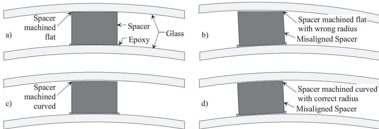
Figure 3. a) The spacer is machined flat and tangential to the optic radius when properly aligned. b) A misalignment in the spacer will cause the spacer to be machined with the wrong radius which may lead to an in-phase roundness error in the mounted shell. c) A spacer is machined uniformly to the correct radius. d) A misalignment in the spacer will have no effect on the spacer performance if the spacer is machined uniformly to the correct radius.
