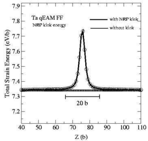
Figure 12: PLN and NRP kinks in Ta using the qEAM FF. (Top Left) PLN kink: Dislocation position in the [11-2] direction along the dislocation line; we can see the dislocation moves from one equilibrium position to the next in a distance of 10 Burgers vectors. (Top Right) PLN kink: total energy in the quadrupolar system with four PLN kinks along the dislocation line. The system is divided in slices with thickness equal to b and the energy in each region is calculated. (Bottom Left) NRP kink: Dislocation position in the [11-2] direction along the dislocation line; we can see the dislocation moves from one equilibrium position to the next in a distance of 10 Burgers vectors. (Bottom Right) NRP kink: total energy in the quadrupolar system with four PLN kinks along the dislocation line.
