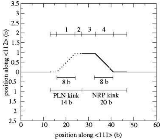
Figure 13: Schematic diagram of a kink pair formed by a NRP and PLN single kinks. The four terms entering in the work expression (Equation 16) are shown in the Figure.
