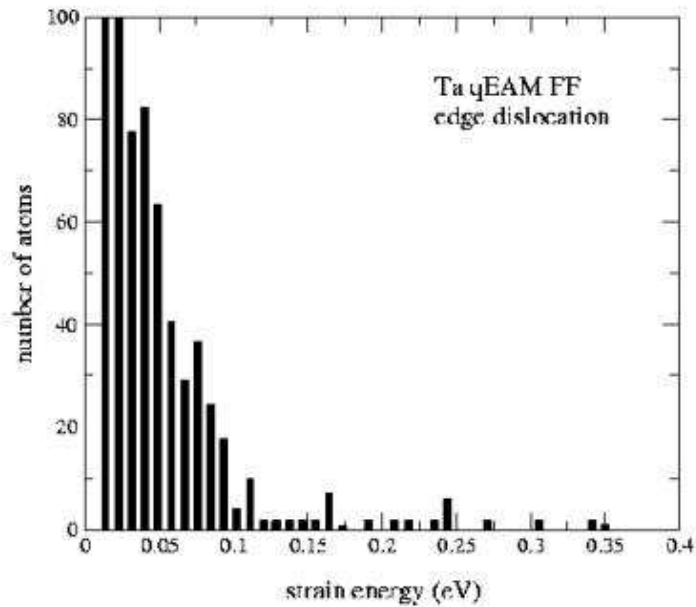
Figure 11: Histogram of atomistic strain energy distribution for the dipole of edge dislocations. The number of atoms is given per dislocation and per 1/2a < 112 > length.
