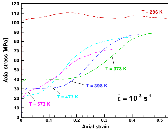
(a) Experimental data of Mitchell & Spitzig [47]
