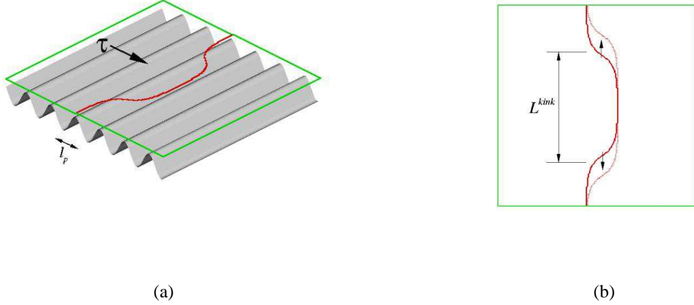
Figure 1: Schematic of the double-kink mechanism.
