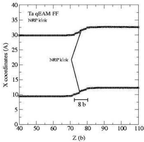
Figure 12: PLN and NRP kinks in Ta using the qEAM FF. (Top Left) PLN kink: Dislocation position in the [11-2] direction along the dislocation line; we can see the dislocation moves from one equilibrium position to the next in a distance of 10 Burgers vectors. (Top Right) PLN kink: total energy in the quadrupolar system with four PLN kinks along the dislocation line. The system is divided in slices with thickness equal to b and the energy in each region is calculated. (Bottom Left) NRP kink: Dislocation position in the [11-2] direction along the dislocation line; we can see the dislocation moves from one equilibrium position to the next in a distance of 10 Burgers vectors. (Bottom Right) NRP kink: total energy in the quadrupolar system with four PLN kinks along the dislocation line.
