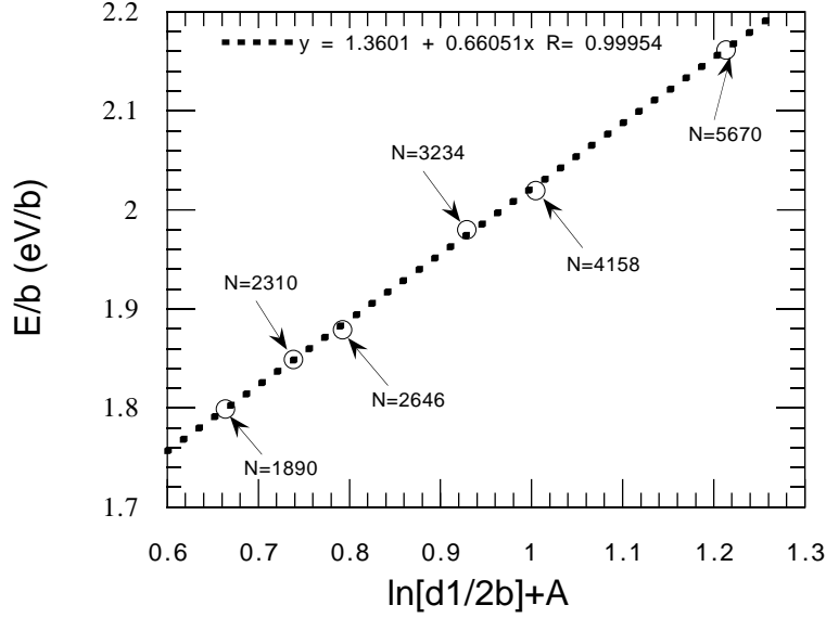
Figure 8: Total strain energy of the quadrupolar system as a function of \ln d_1/r_c + A(d_1/d_2) ; the number of atoms in each simulation is shown. The dashed line is the linear fit to our atomistic data.
