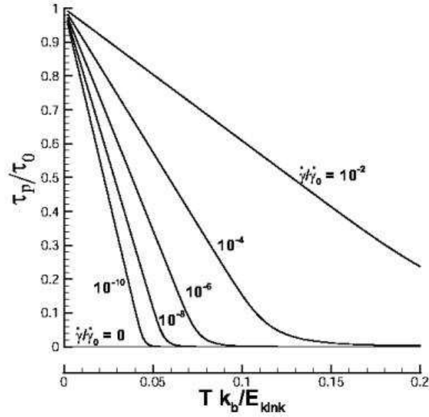
Figure 2: Temperature dependence of the effective Peierls stress for various strain rates. Note that the typical order of magnitude of \dot{\gamma}_0^{\text{kink}} = 10^6 \text{ s}^{-1} .
